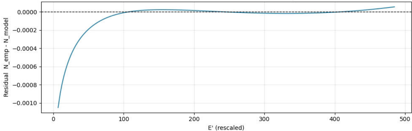
Proof 17 — Residuals after OT rescaling
