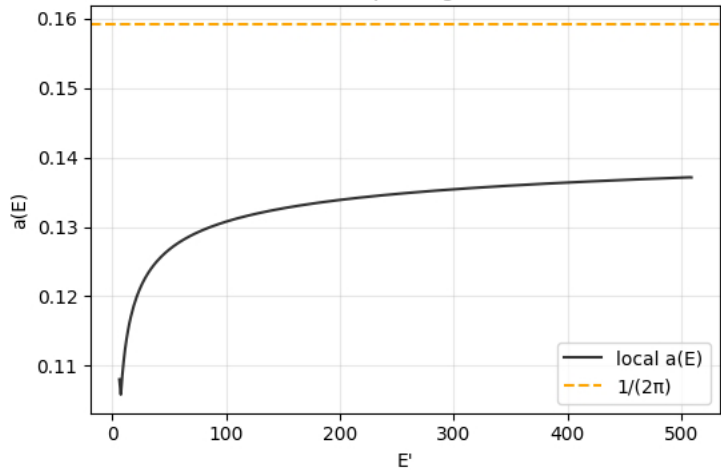
Local slope diagnostics
