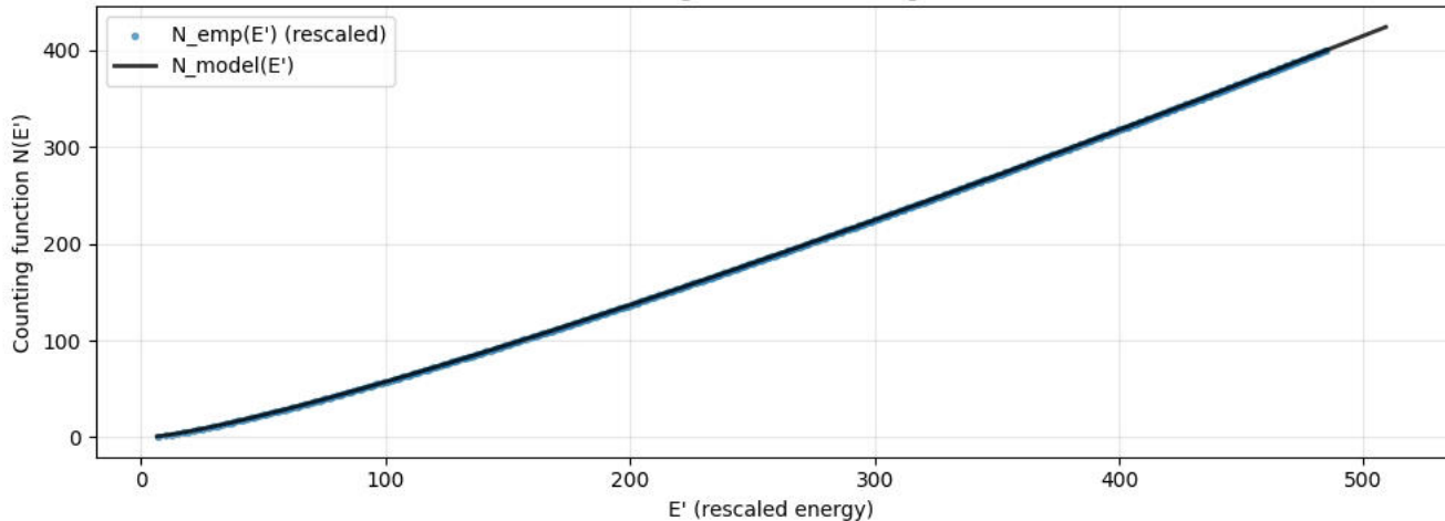
Proof 17 — Counting after OT rescaling ( \lambda=0.159145 )
