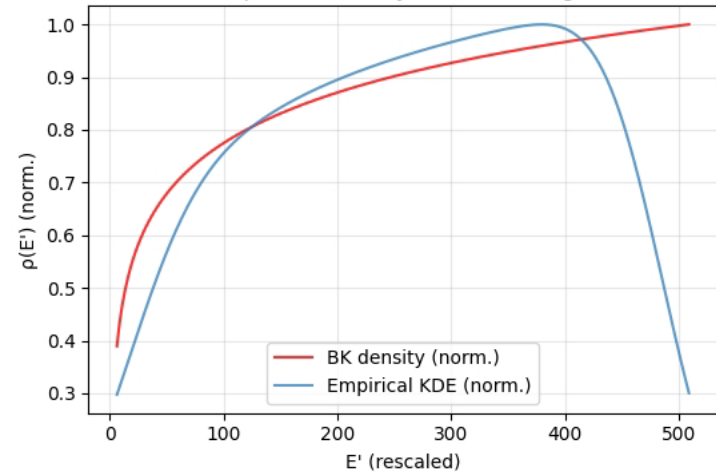
Spectral density after rescaling
