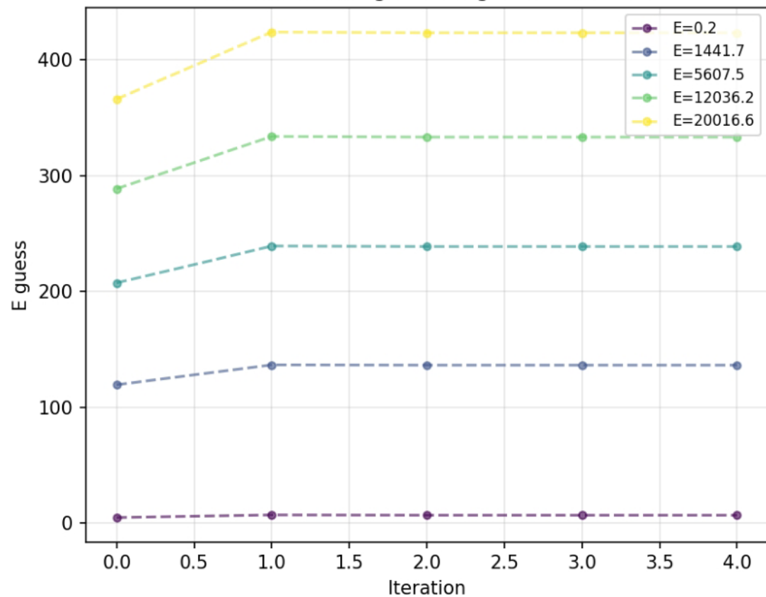
Newton Convergence: E guess evolution
