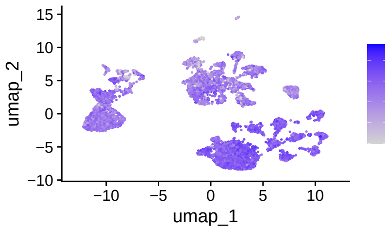
HLA-DQB1
