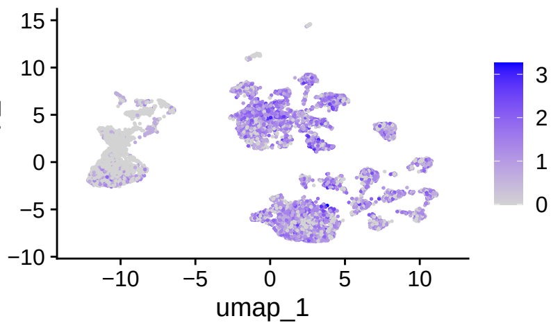
CCR7
