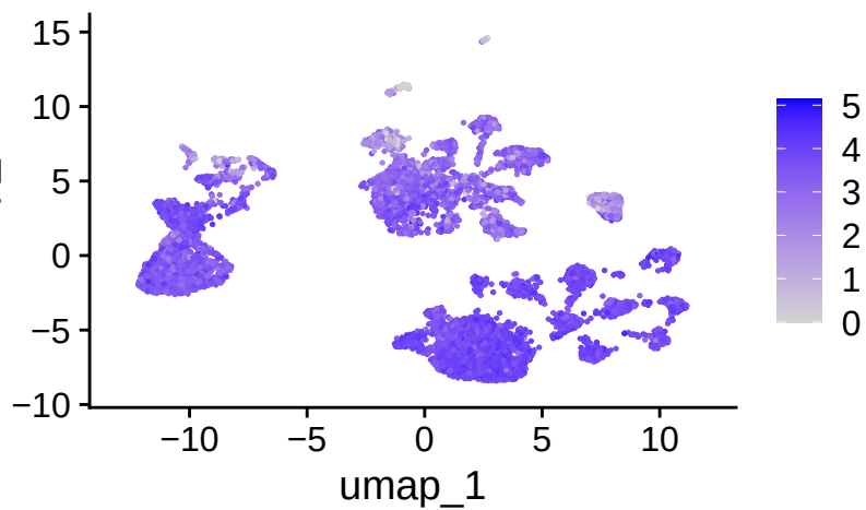
HLA-DPB1
