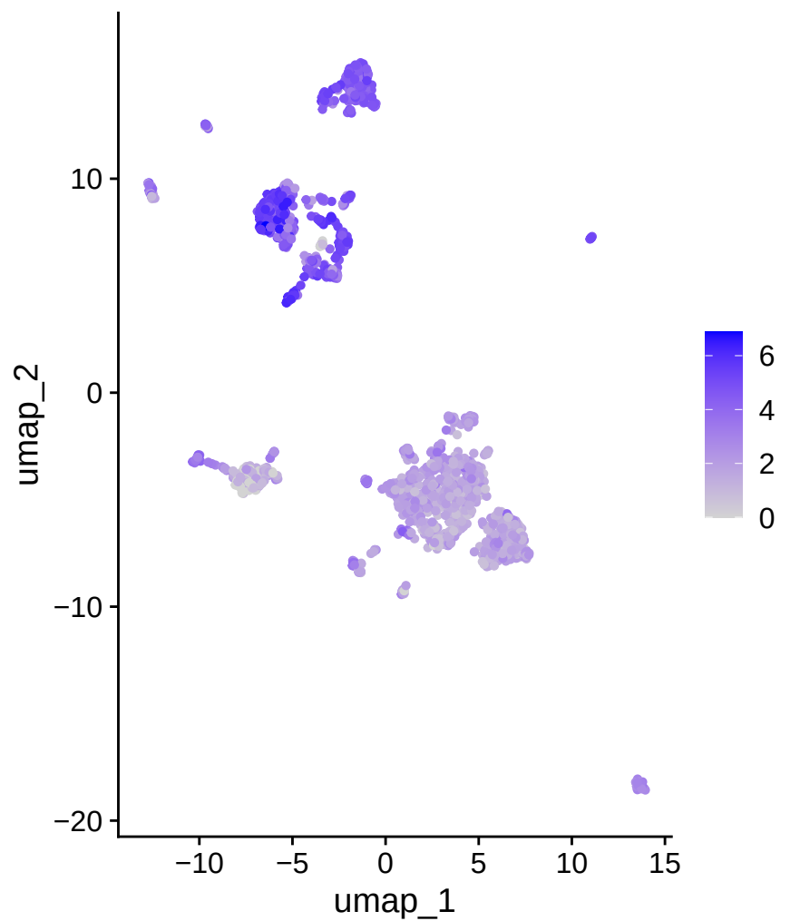
CD74
