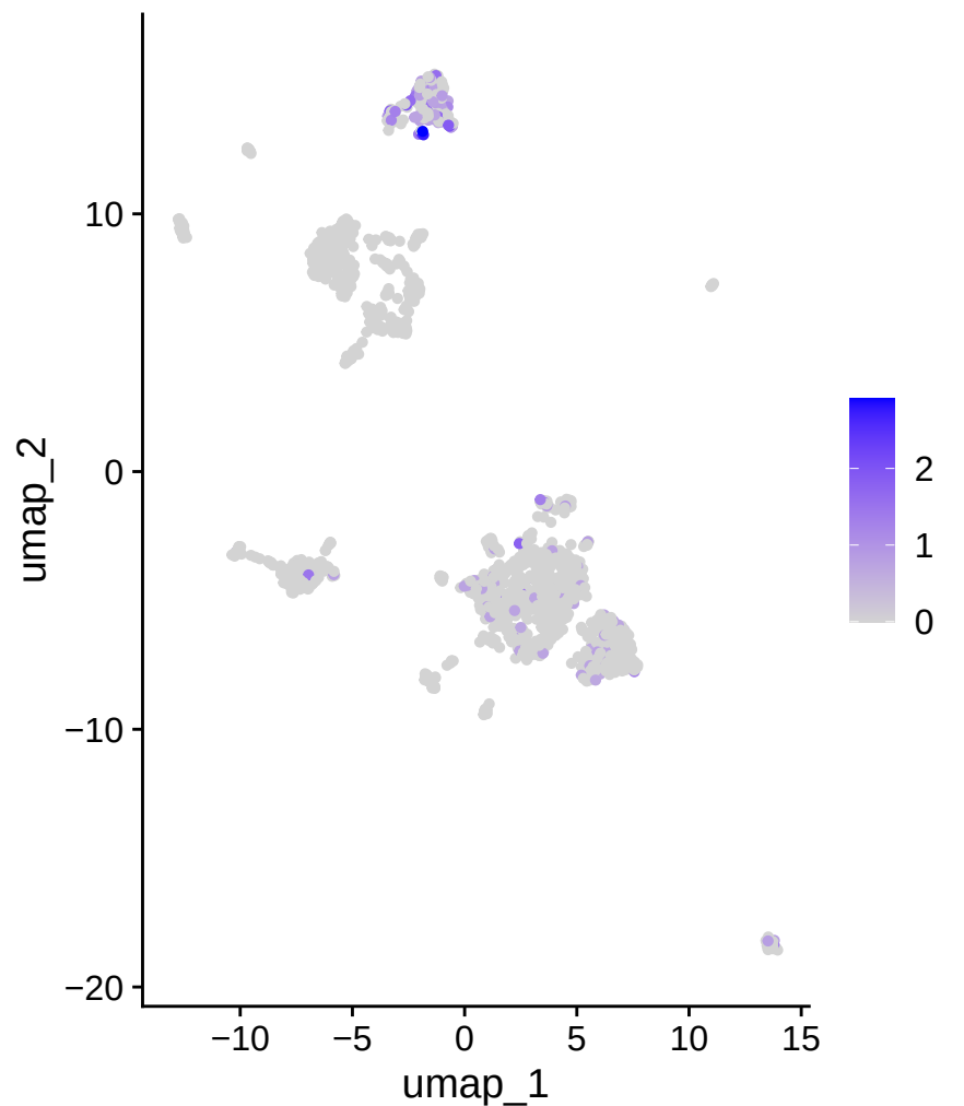
CD74
