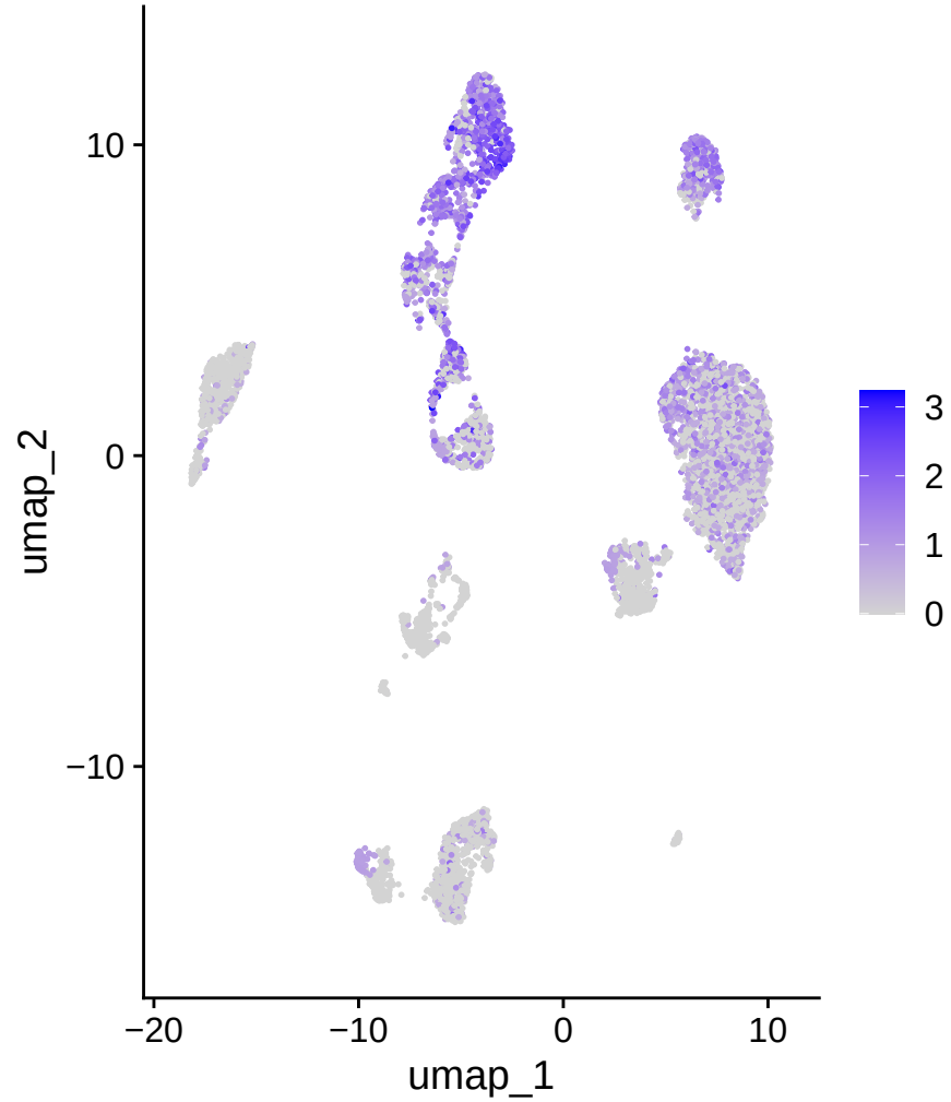
CD74
