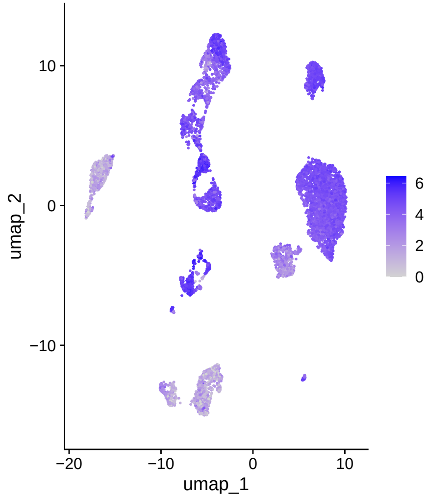
CD74
