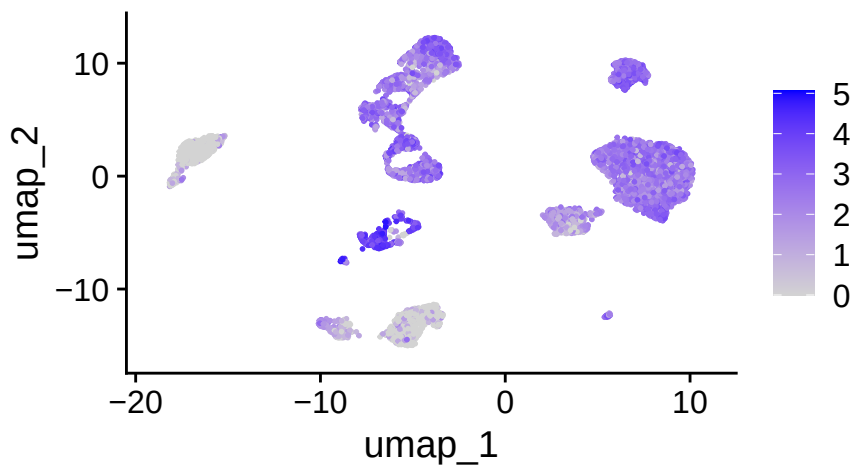
HLA-DQB1
