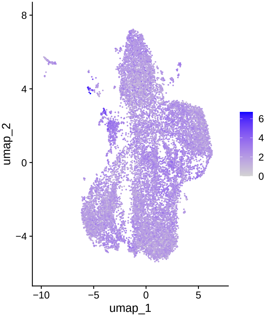
CD74
