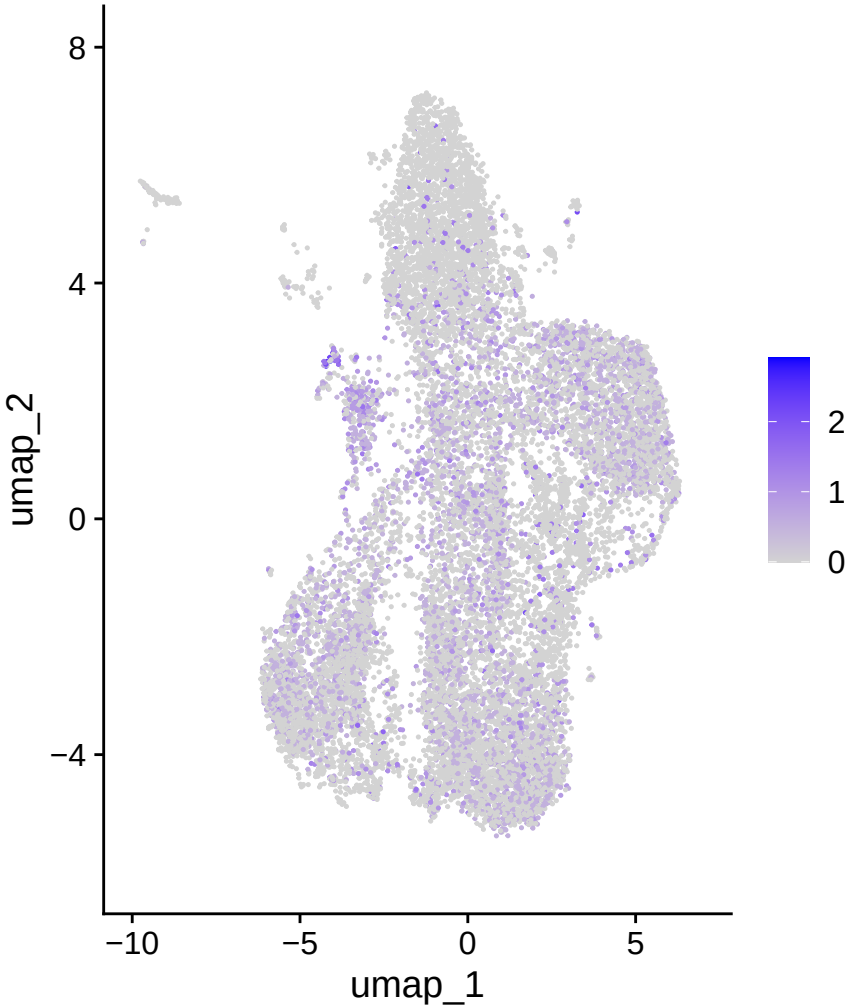
CD74
