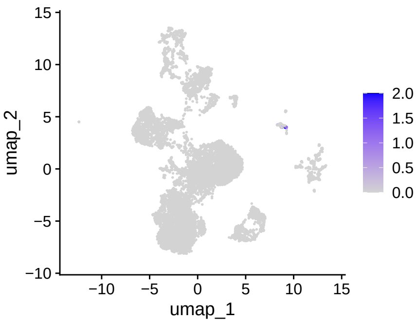
CD7
