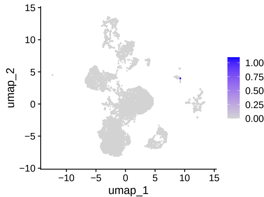
CD8B
