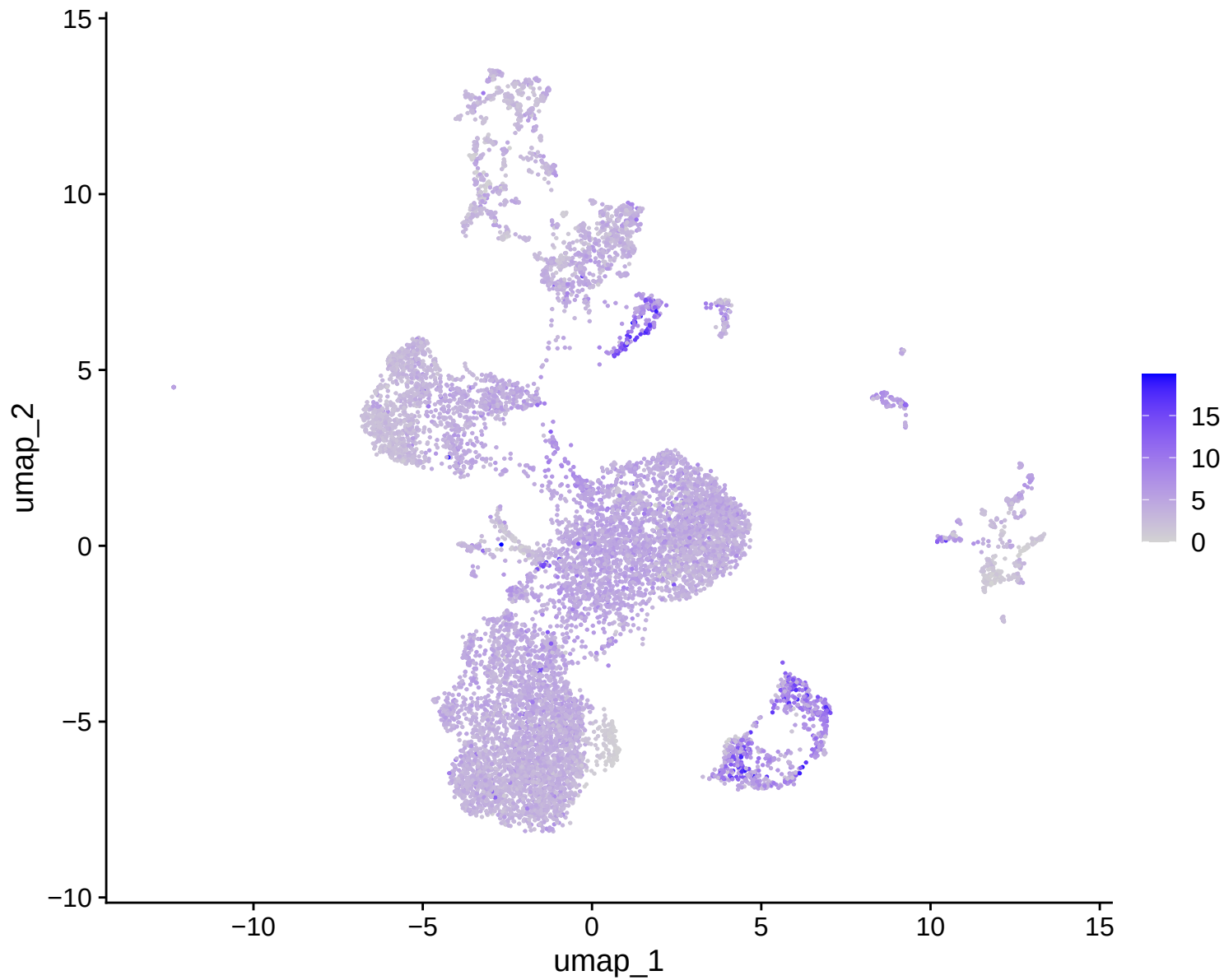
percent.mt
