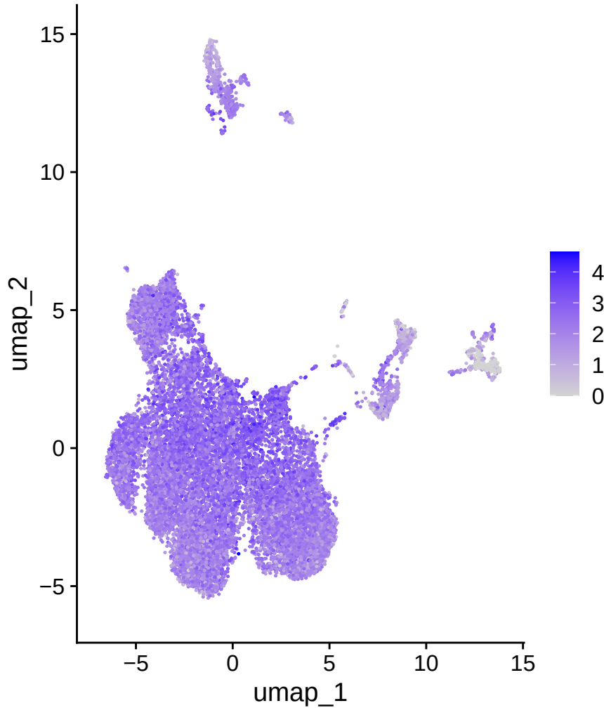
MZB1
