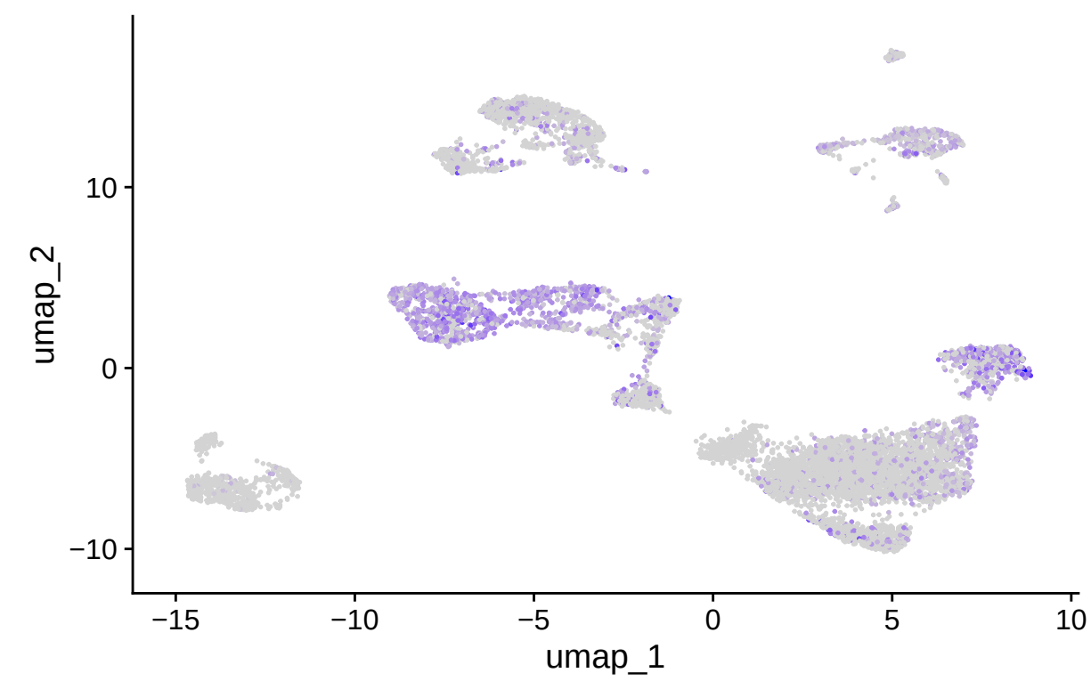
IGHD
