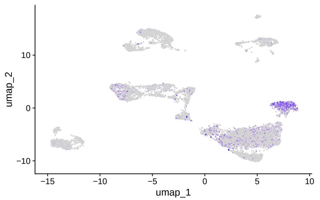
BANK1
