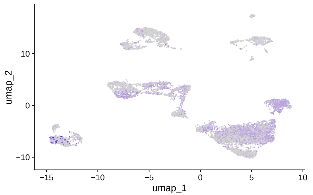
IGHM
