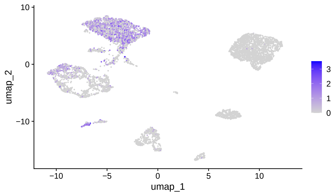
BANK1
