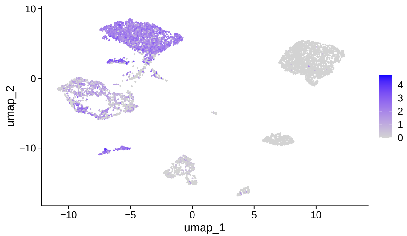
IGHM
