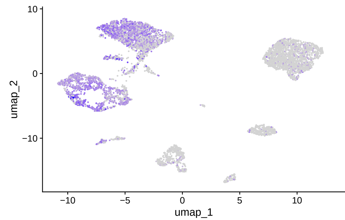
IGHD
