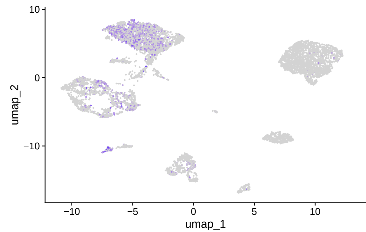
IGHD
