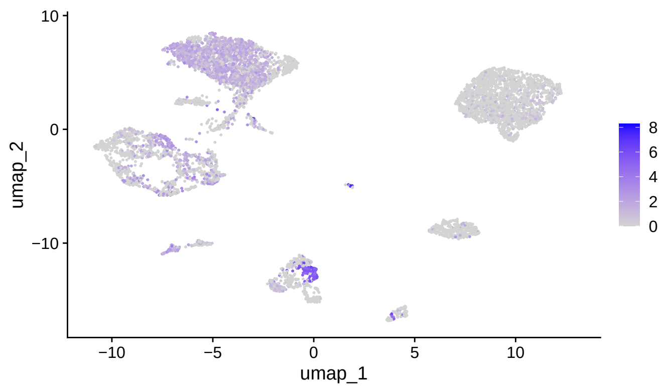
IGHM
