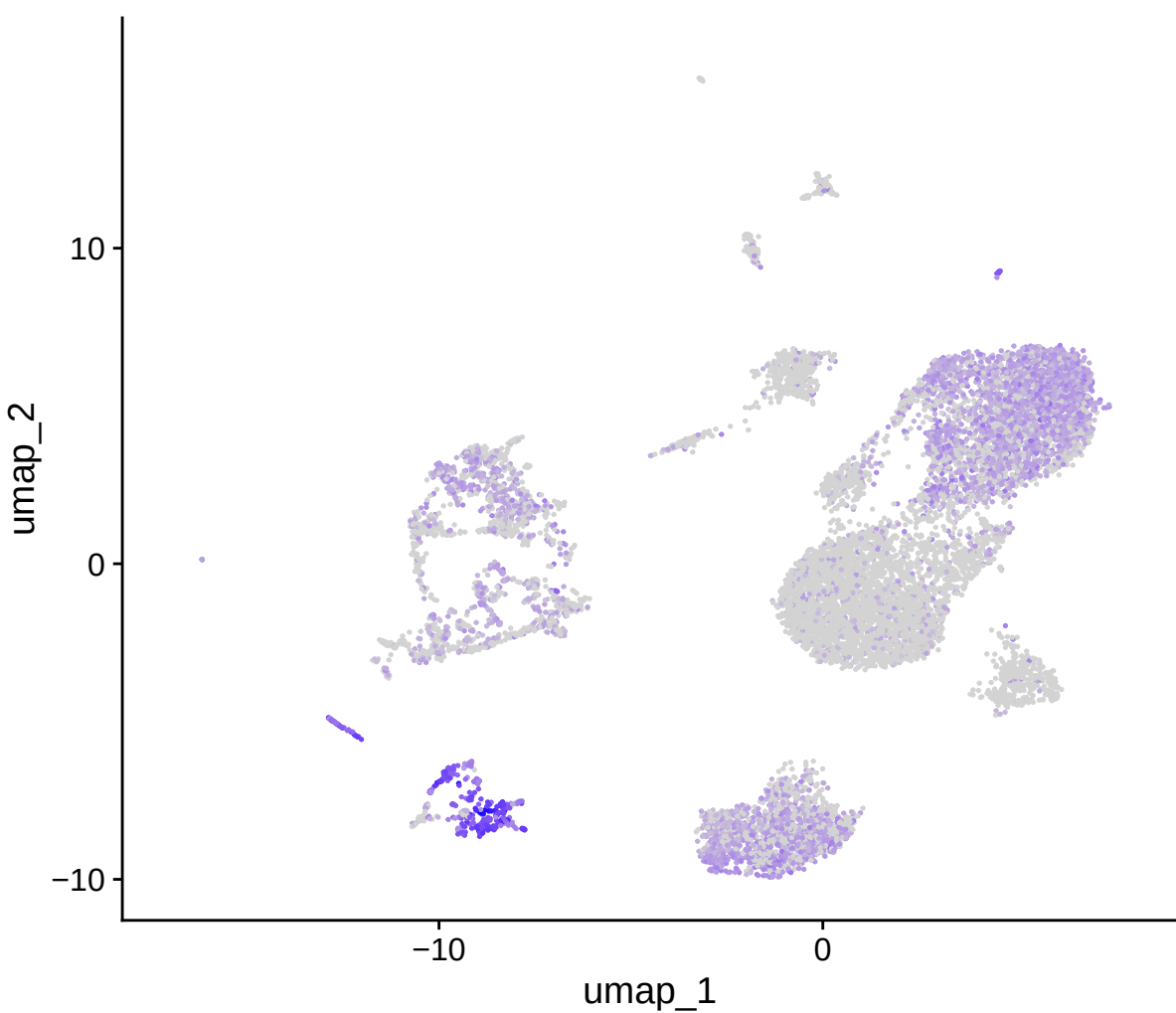
JCHAIN
