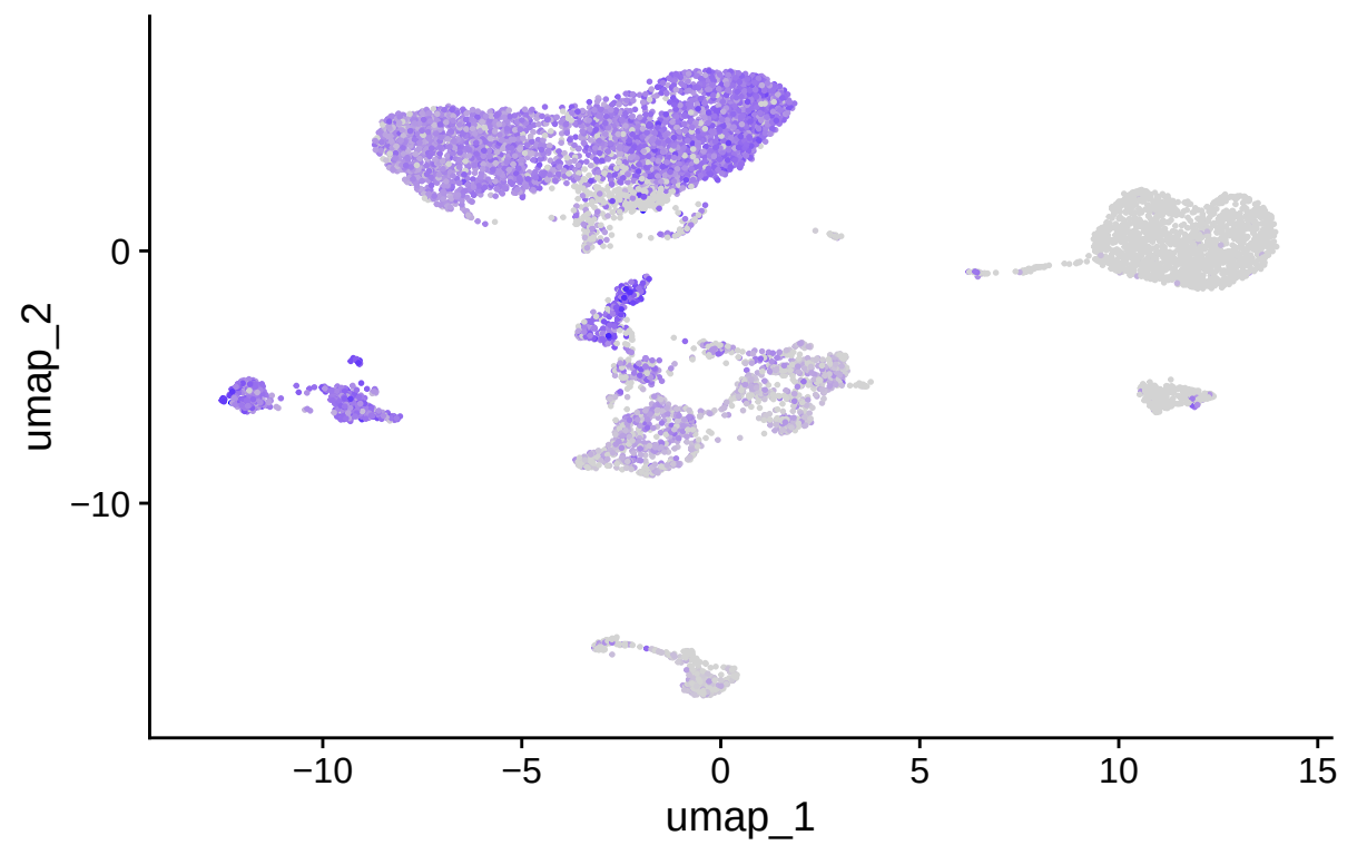
IGHM
