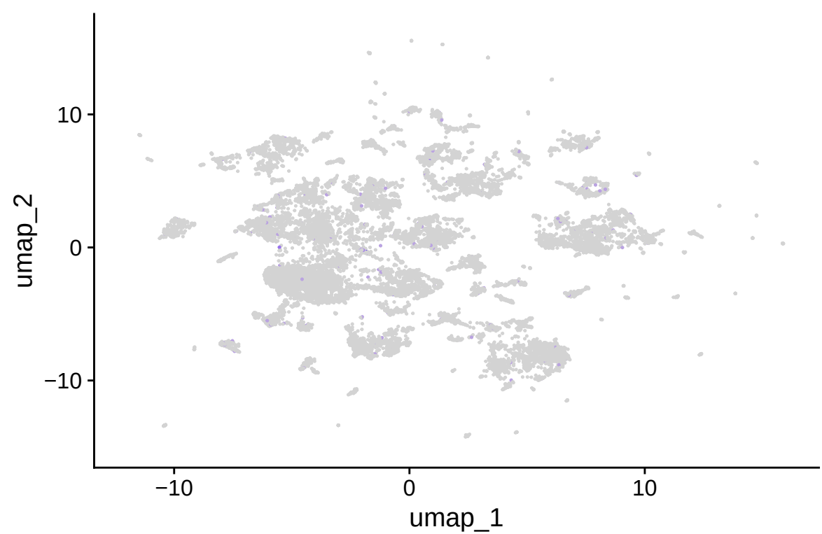
rna_AICDA
