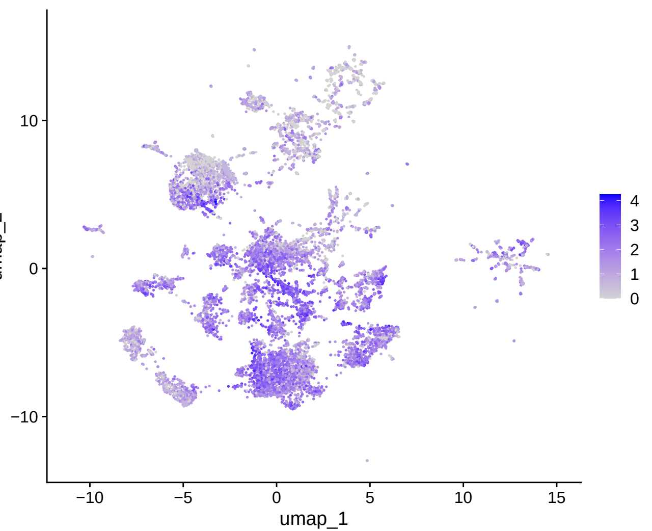
TNFRSF13B
