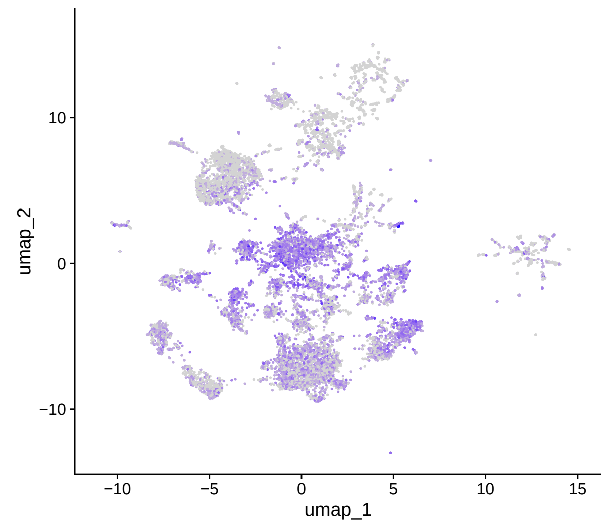
GPR183
