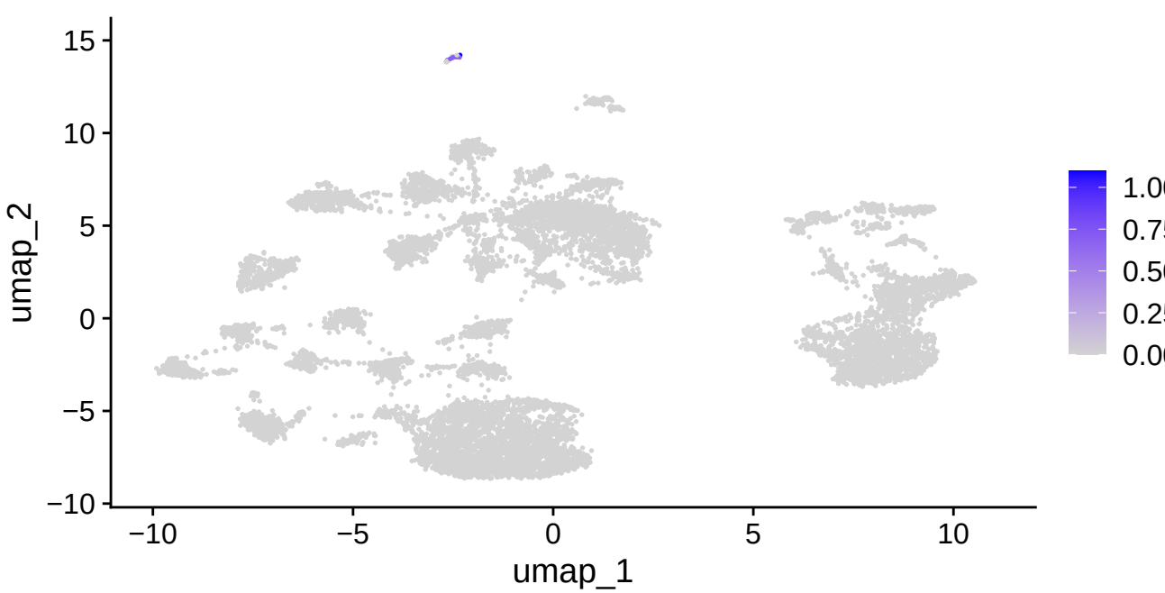
CD3G
