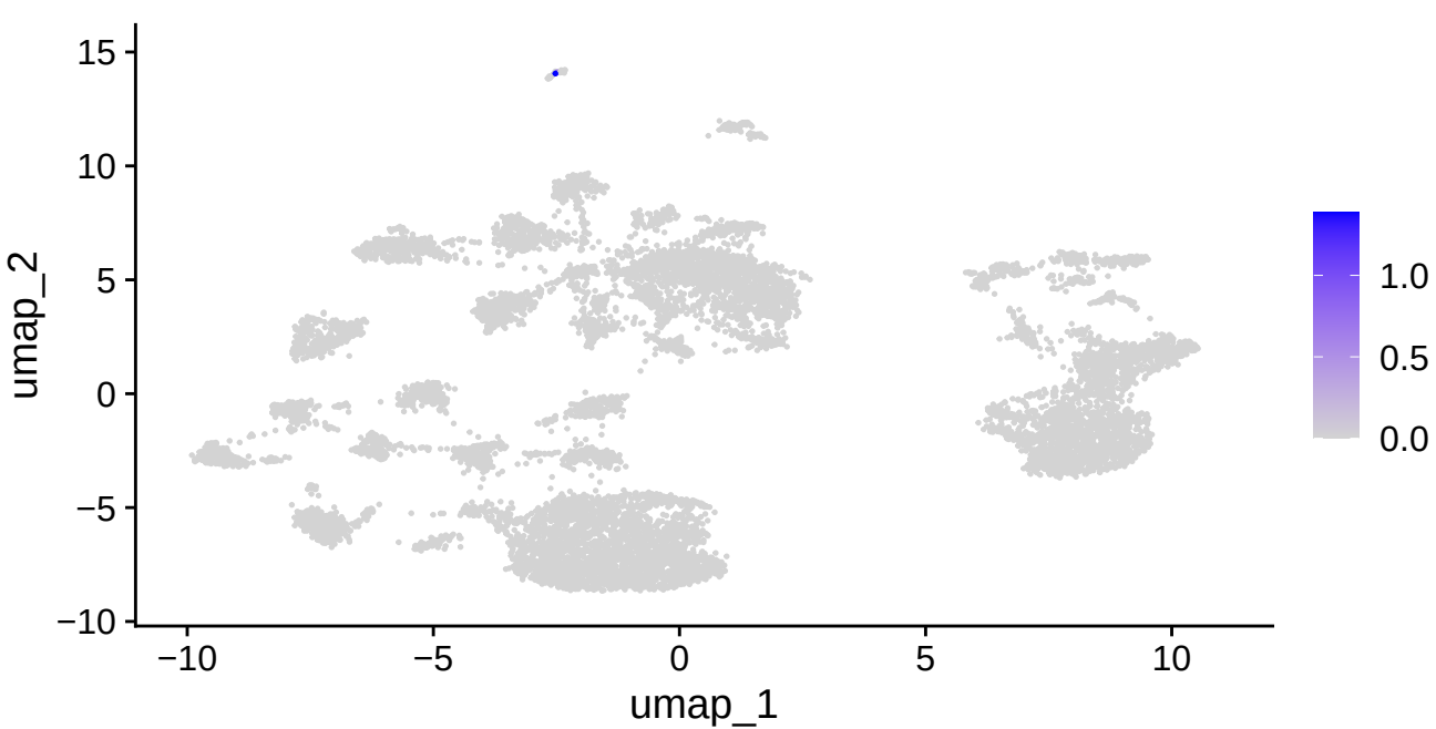
CD8B
