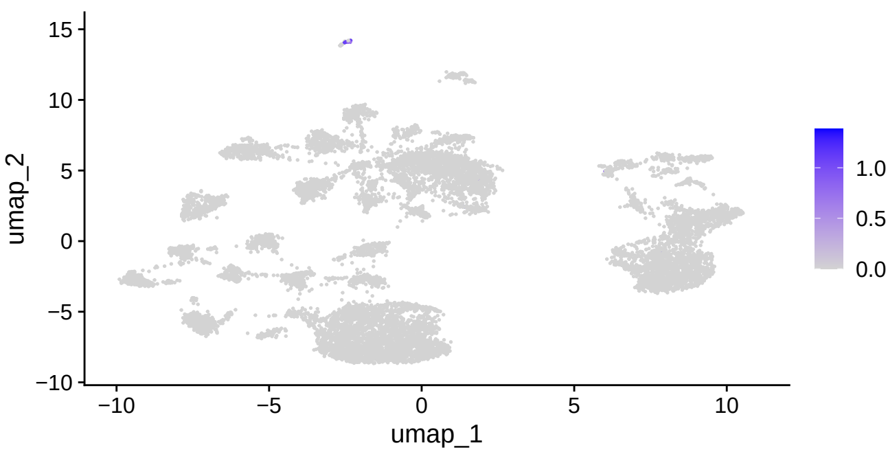
CD3D
