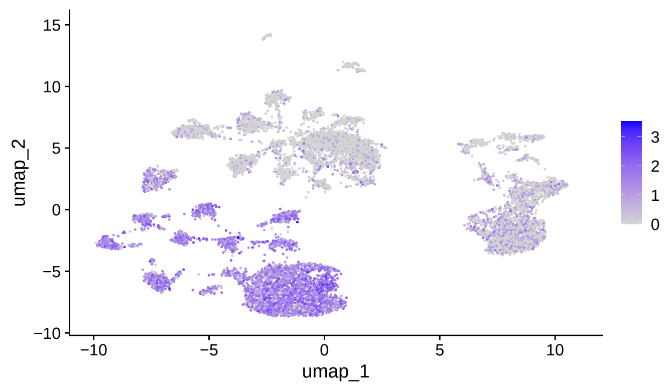
BANK1
