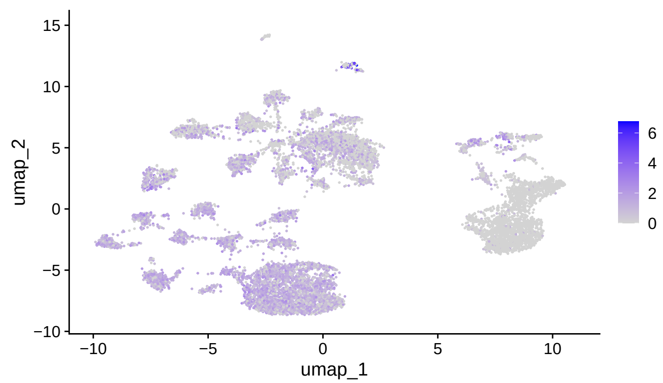
IGHM
