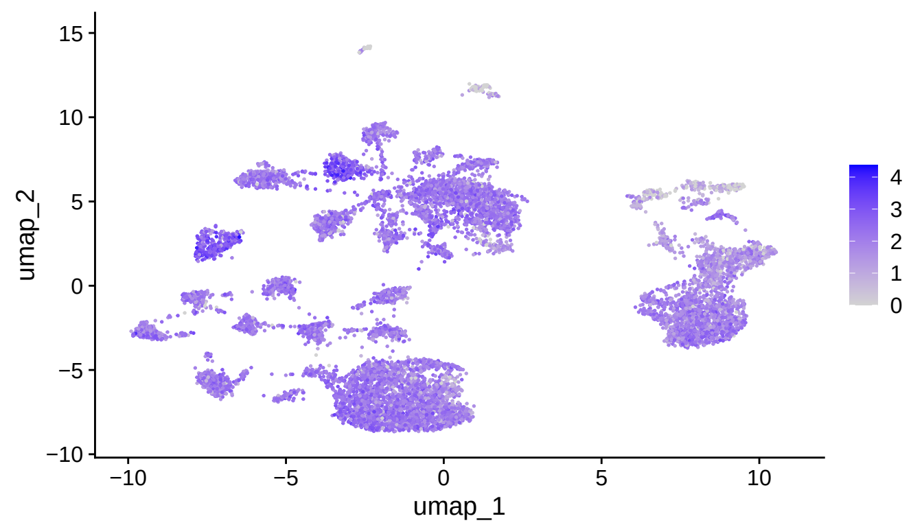
IGHM
