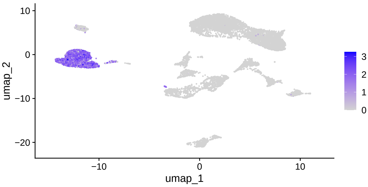
CD3G
