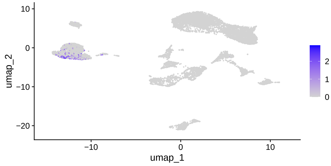
CD8B
