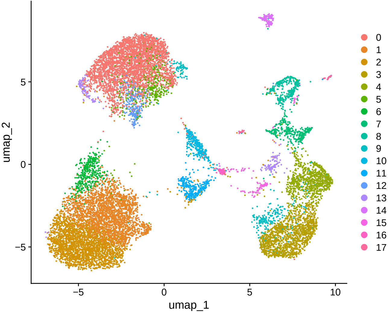
Pre-SoupX
