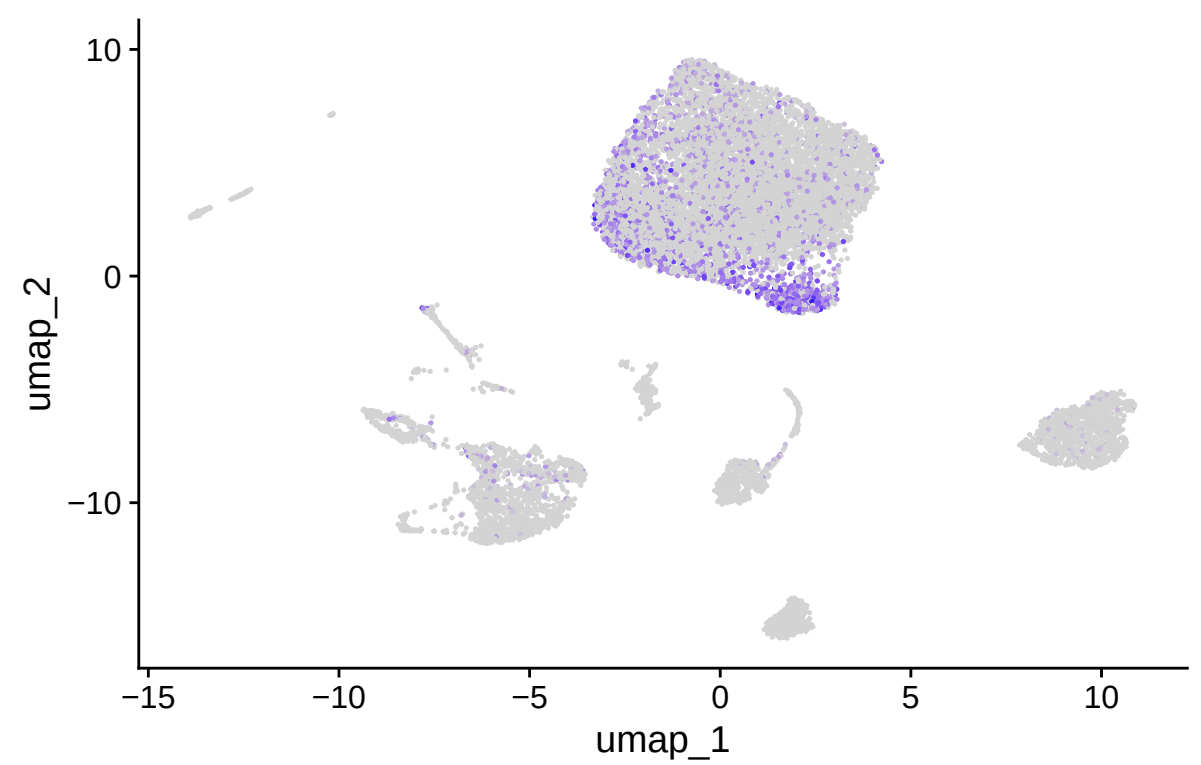
BANK1
