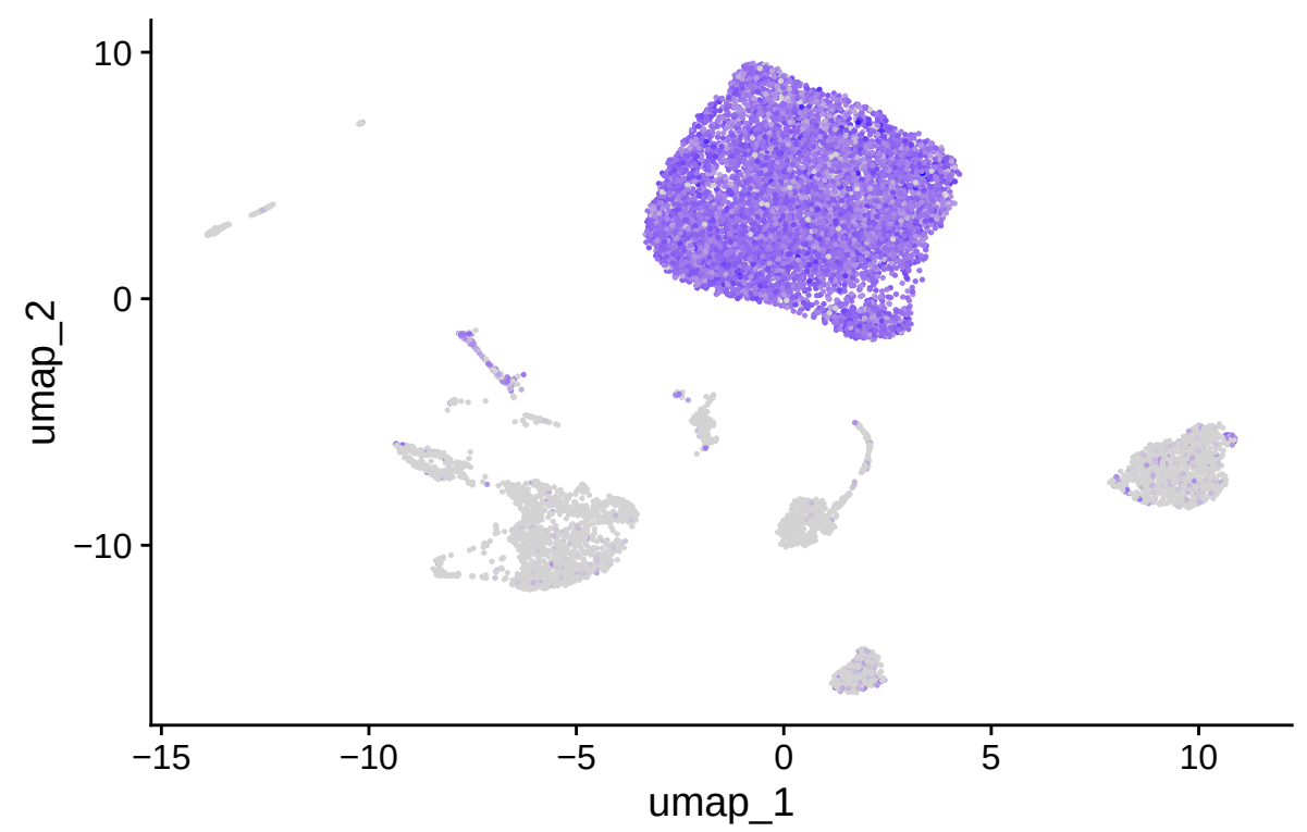
IGHM
