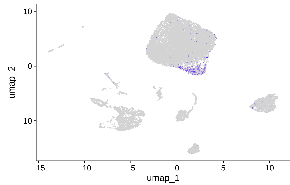
IGHD
