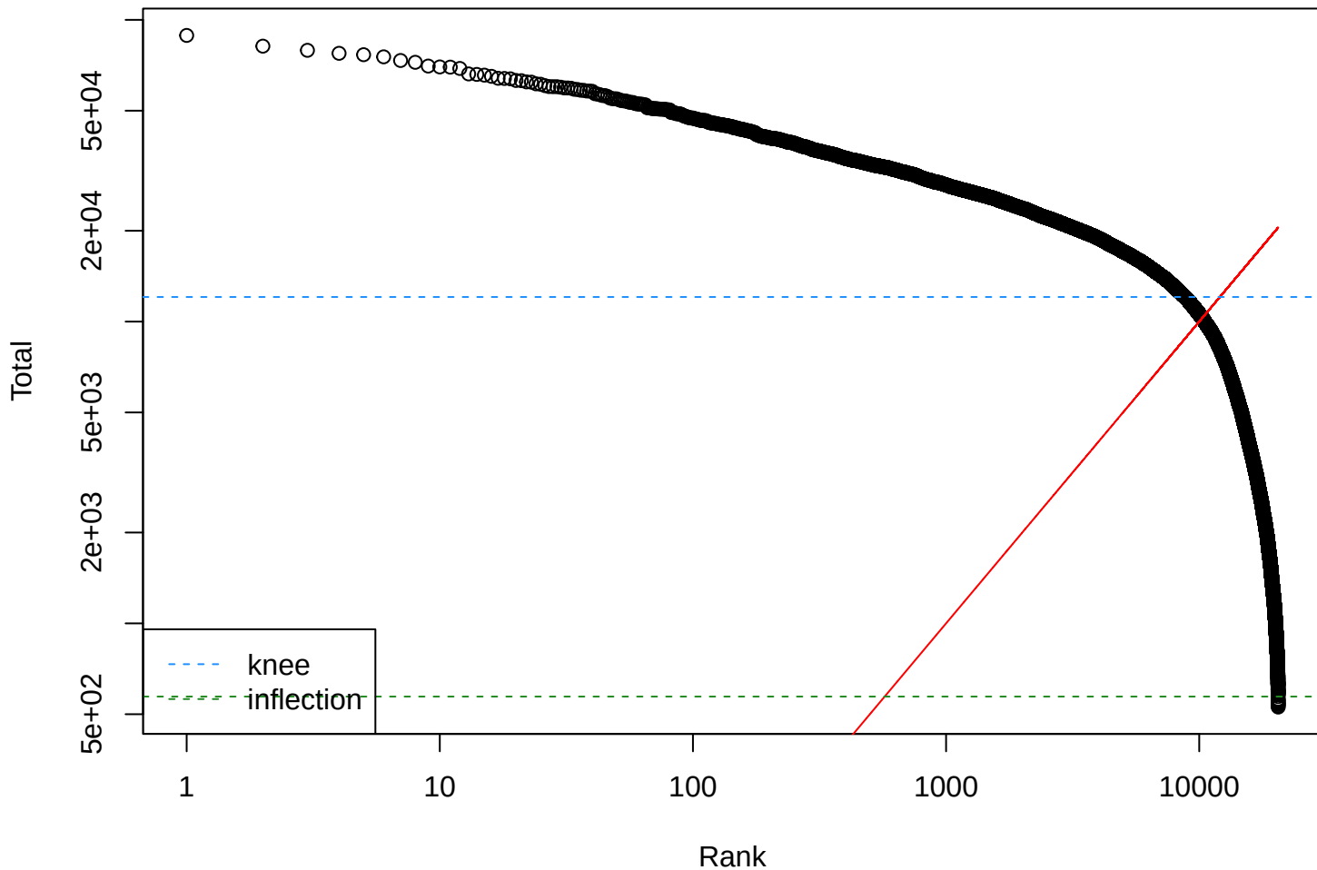
HH119-SILP-PC roughQC-filtered Barcode Rank Plot
