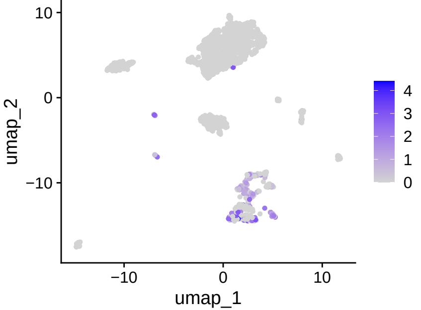
CD7
