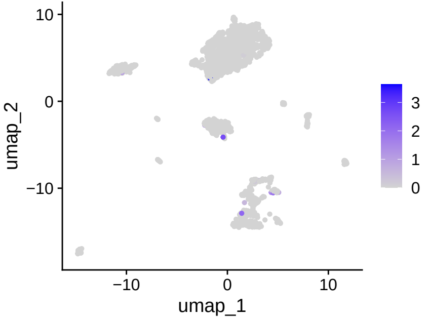
CD7
