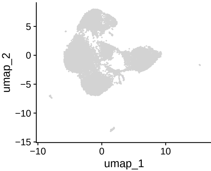
MEF2B
