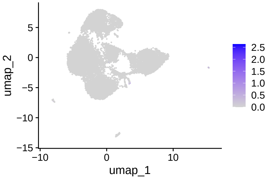
TOP2A
