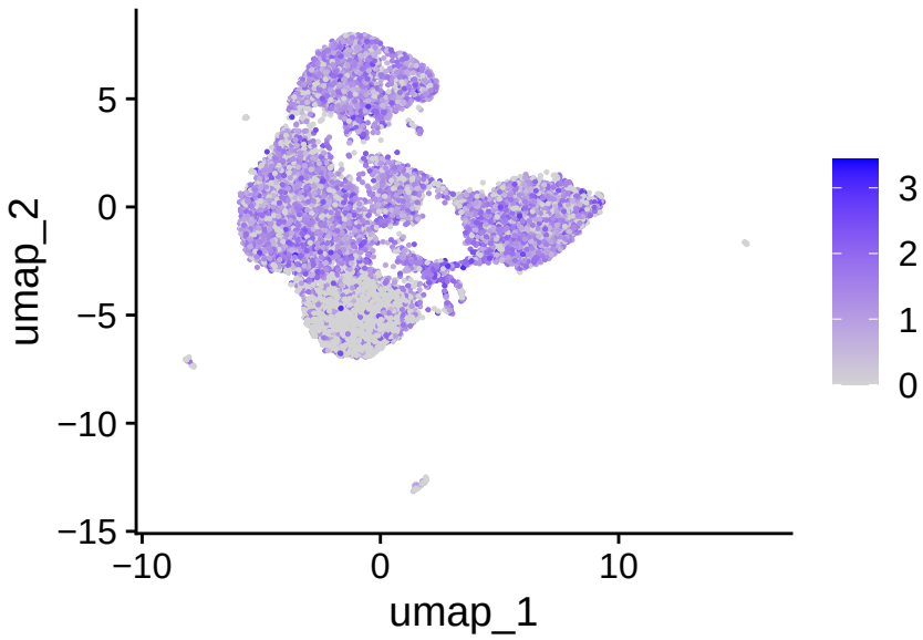
MKI67
