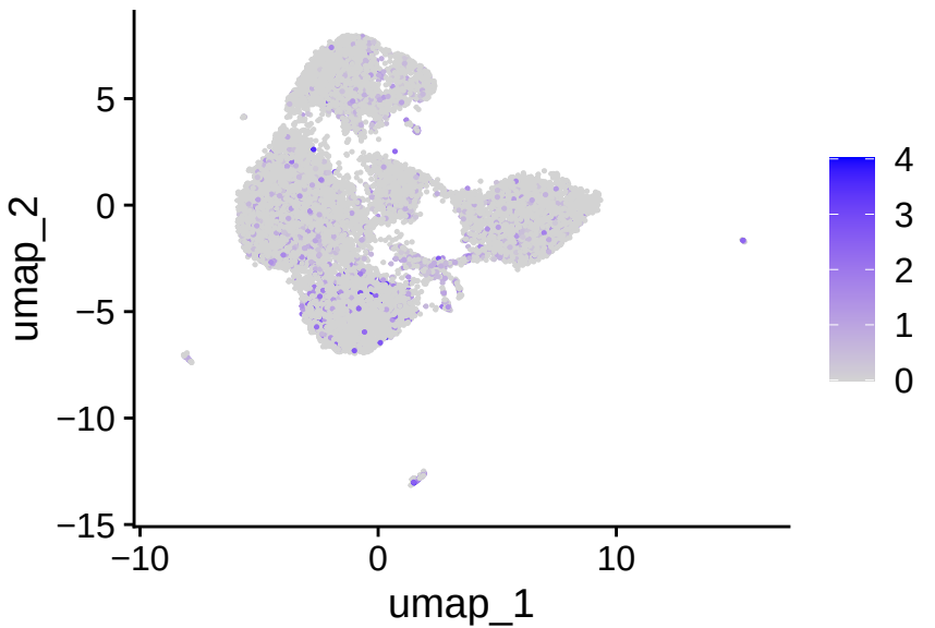
YBX3
