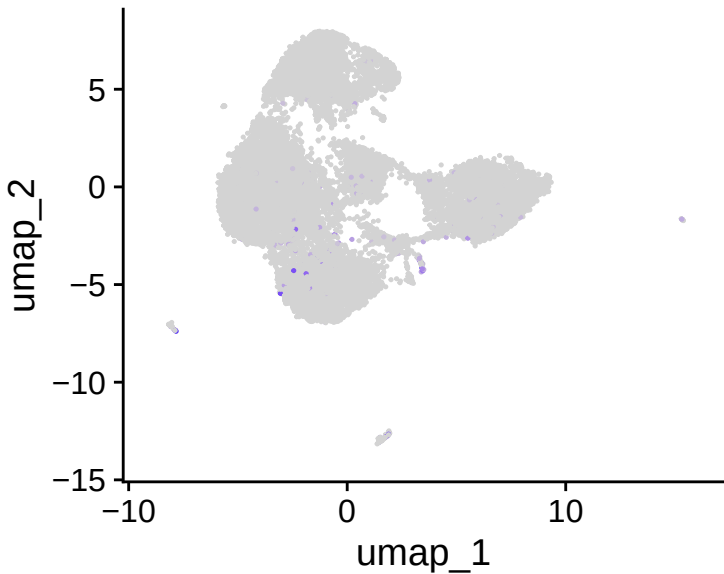
CCR7
