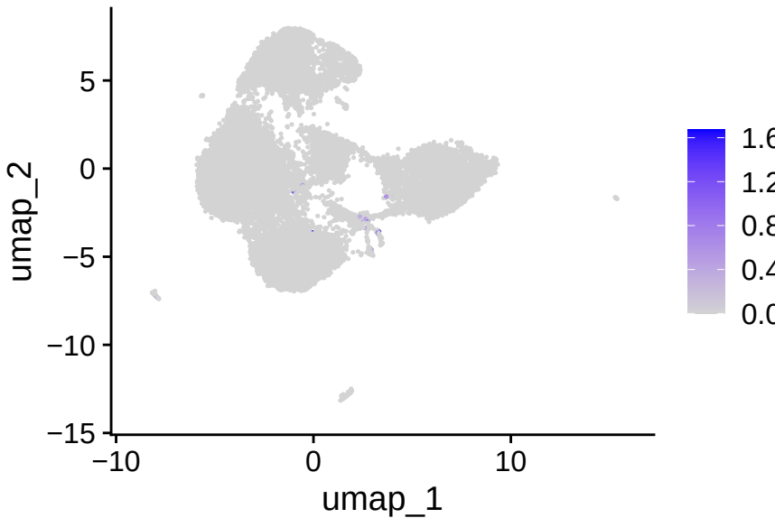
PAX5
