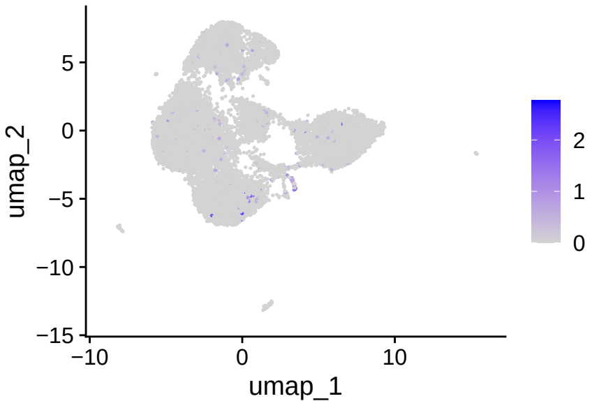
IGHD
