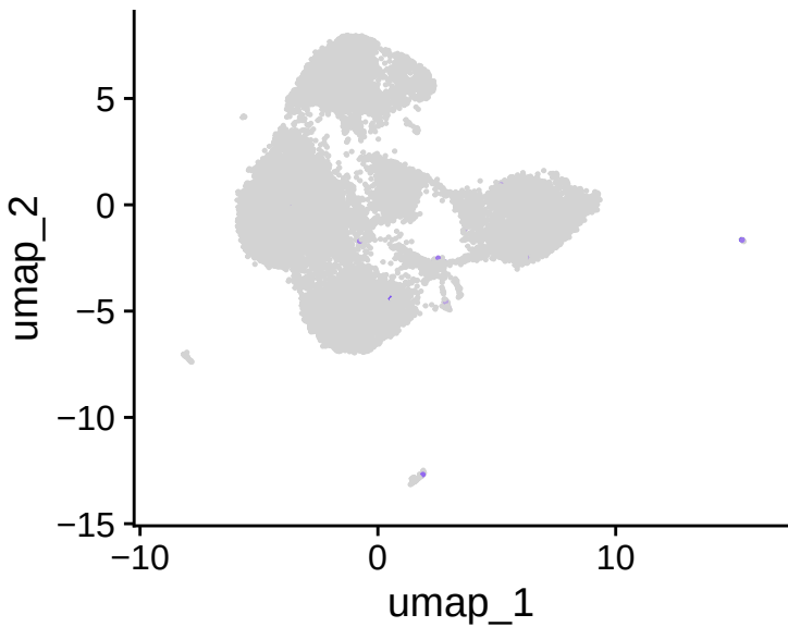
S1PR1
