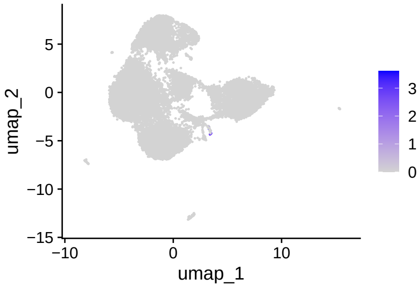
IGHM
