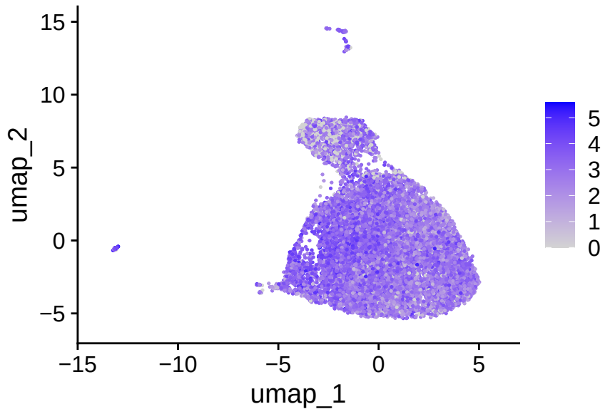
TNFRSF13C
