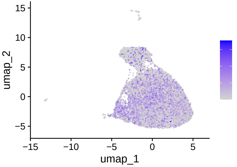
BANK1
