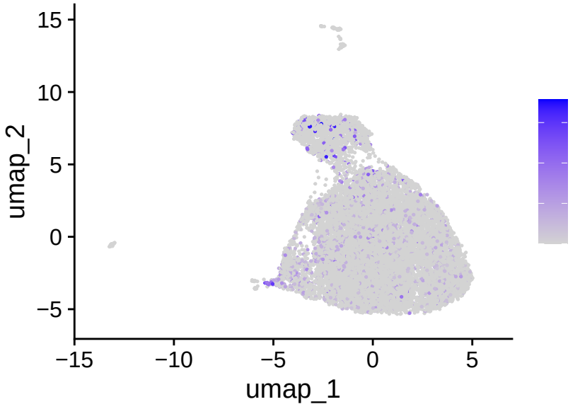
CCR7
