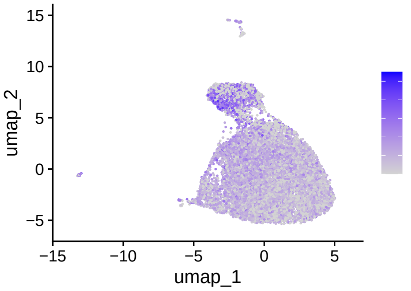
TNFRSF13B
