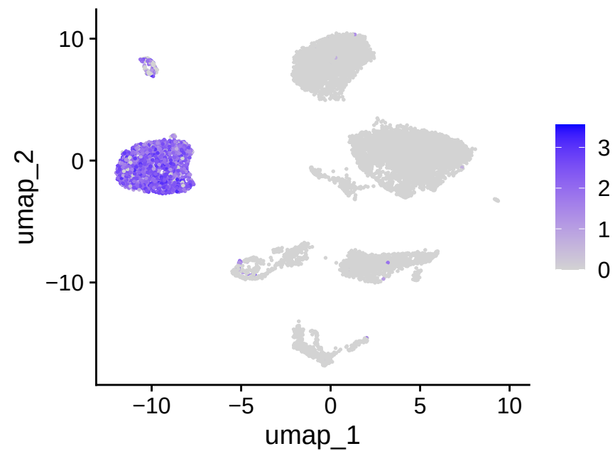
CD8B
