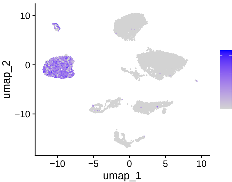
CD7
