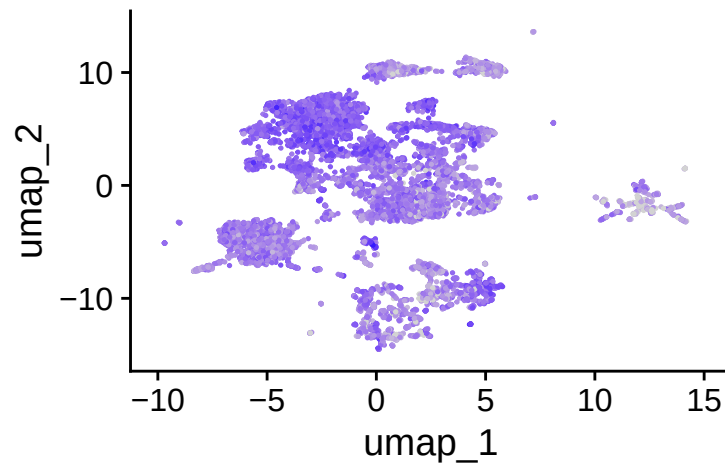
HLA-DQB1
