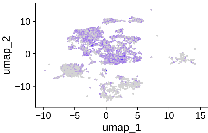
CCR7
