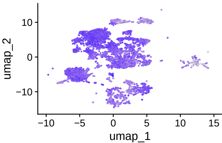
HLA-DPB1
