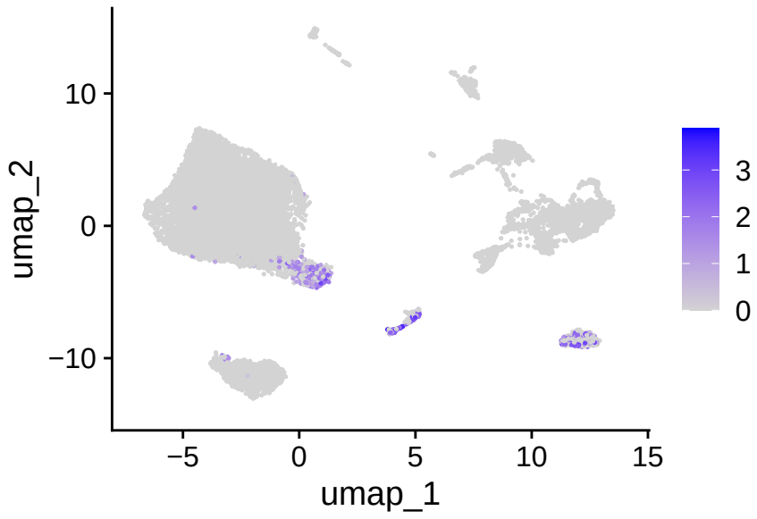
IGHM
