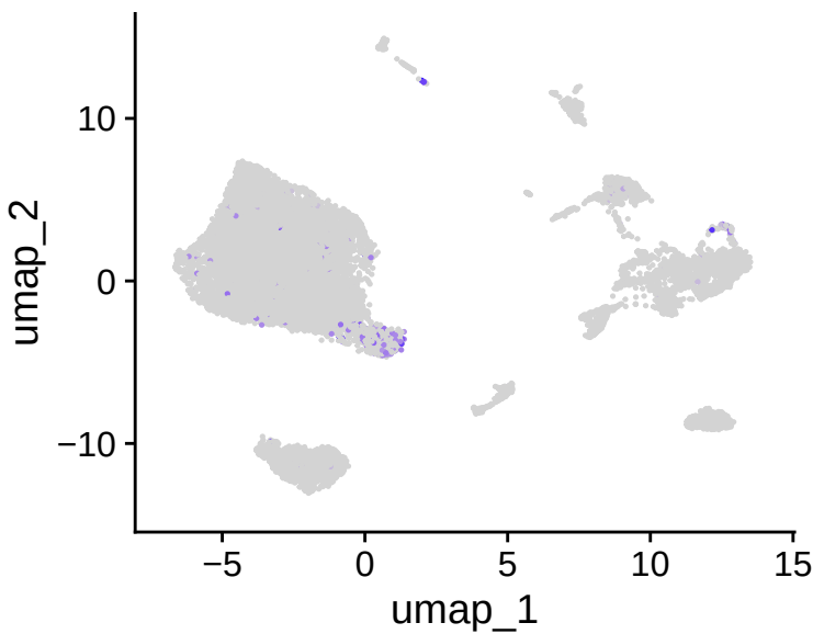
S1PR1
