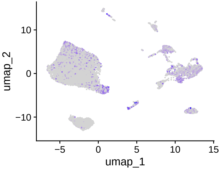
CCR7
