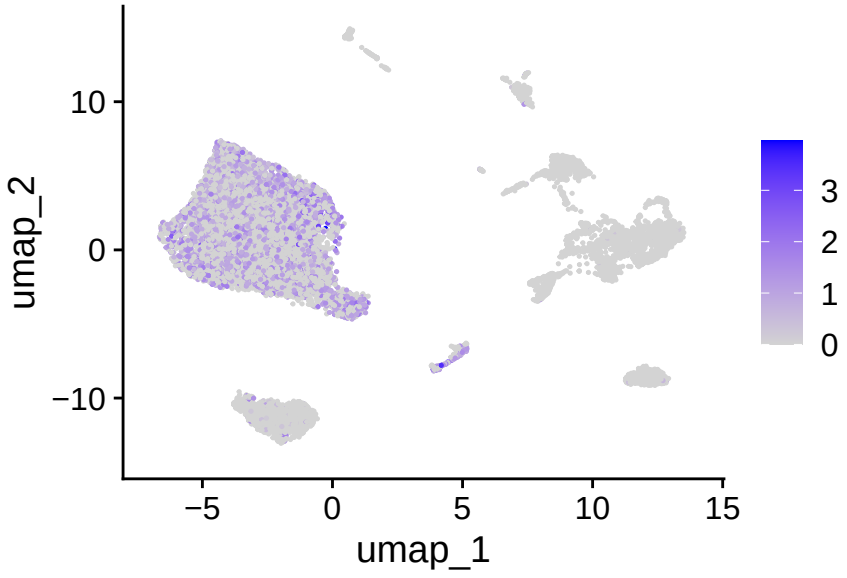
IGHD
