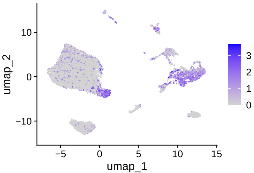
YBX3
