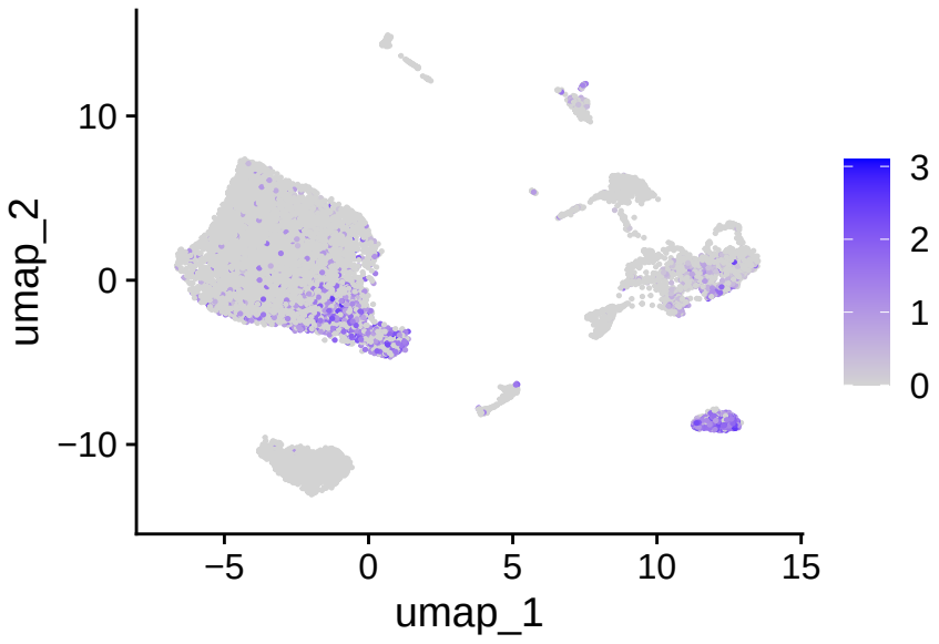
PAX5
