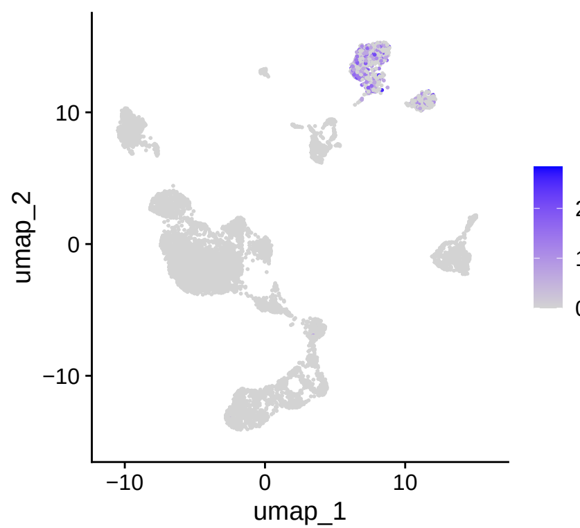
SH2D1A
