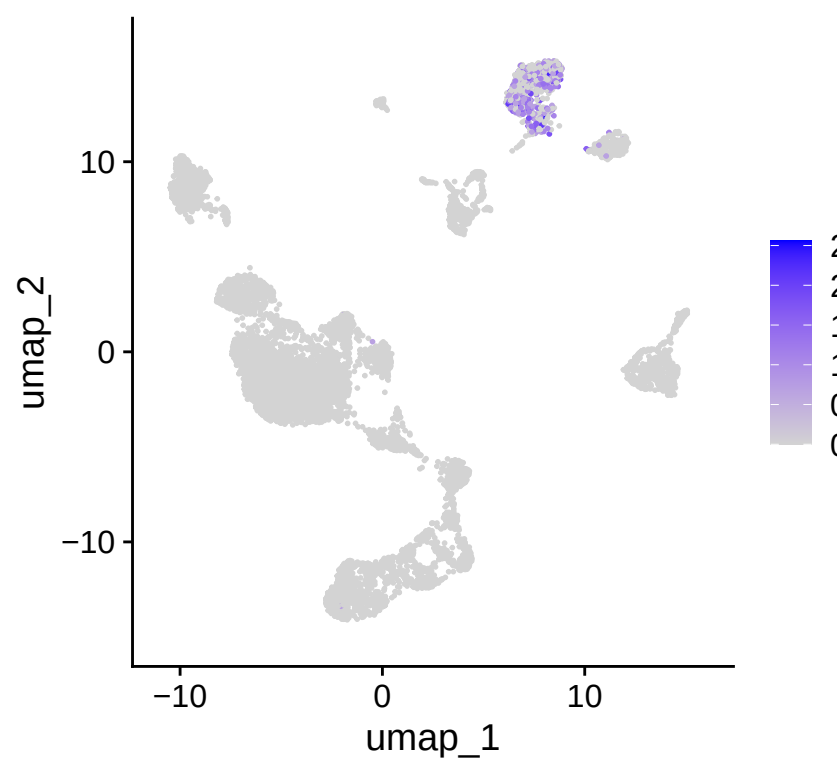
CD84
