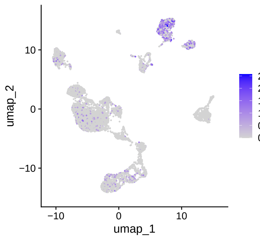
CD84
