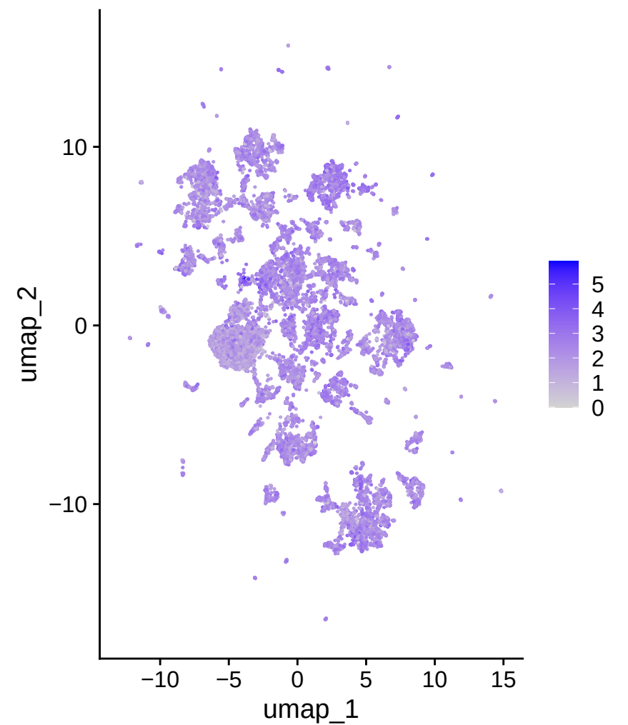
CD74
