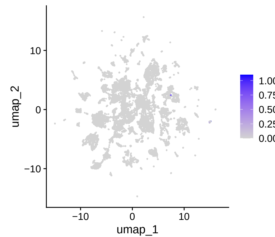
SH2D1A
