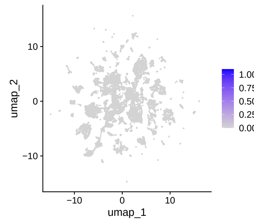
CD84
