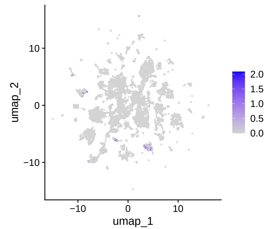
CD84
