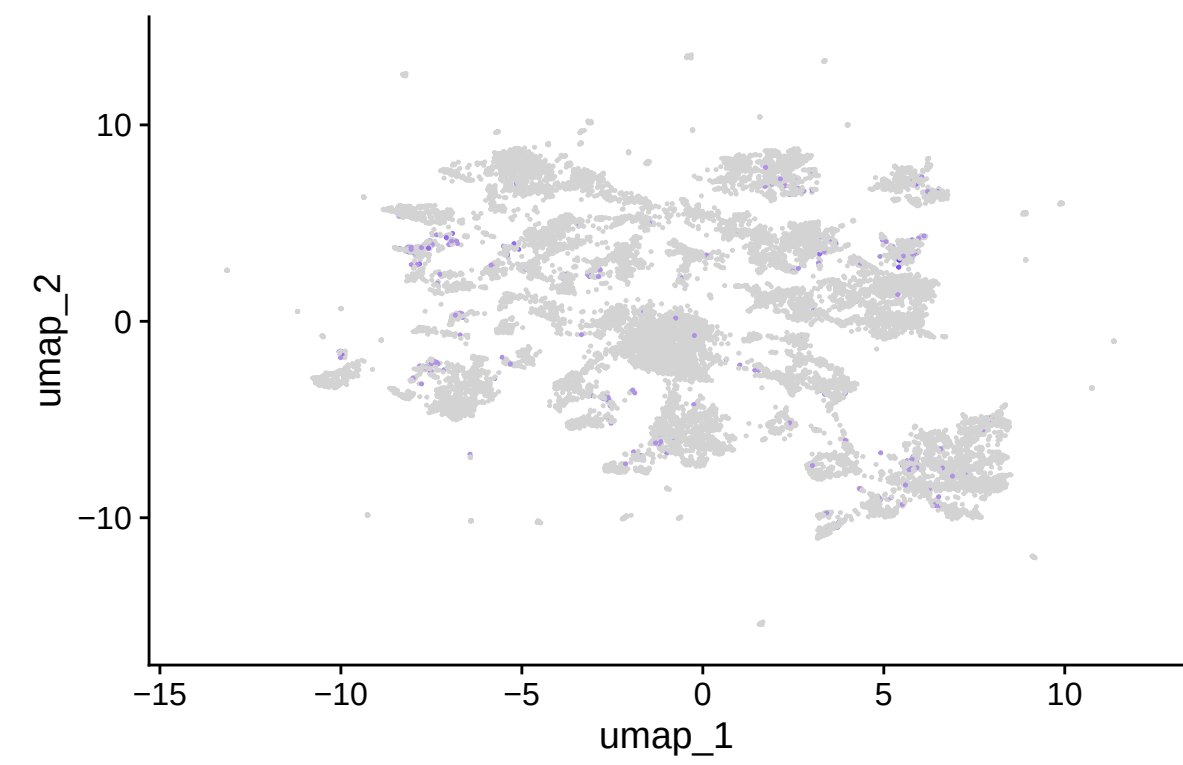
IGHD
