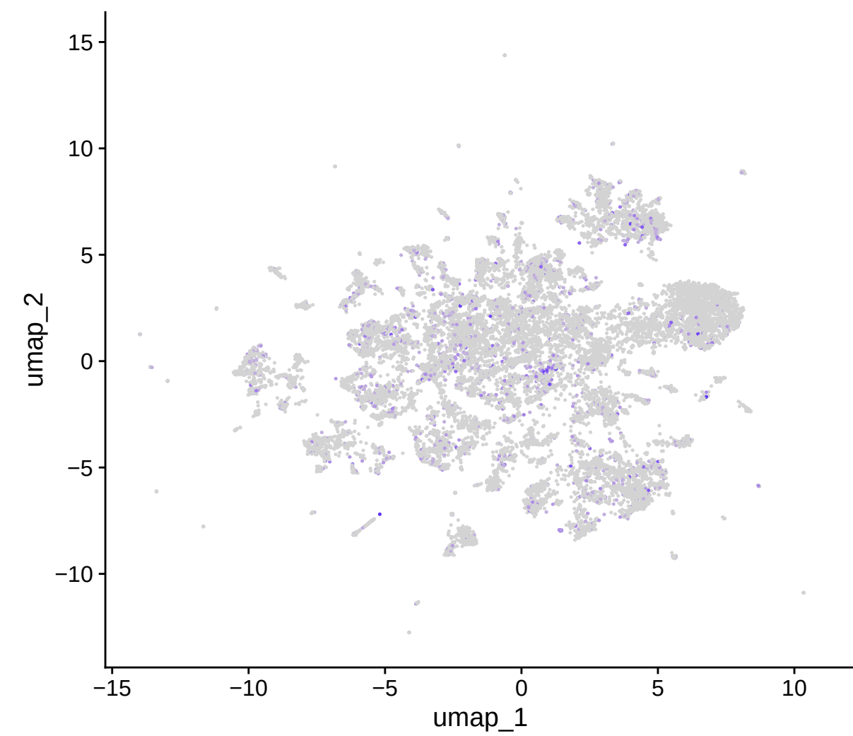
GPR183
