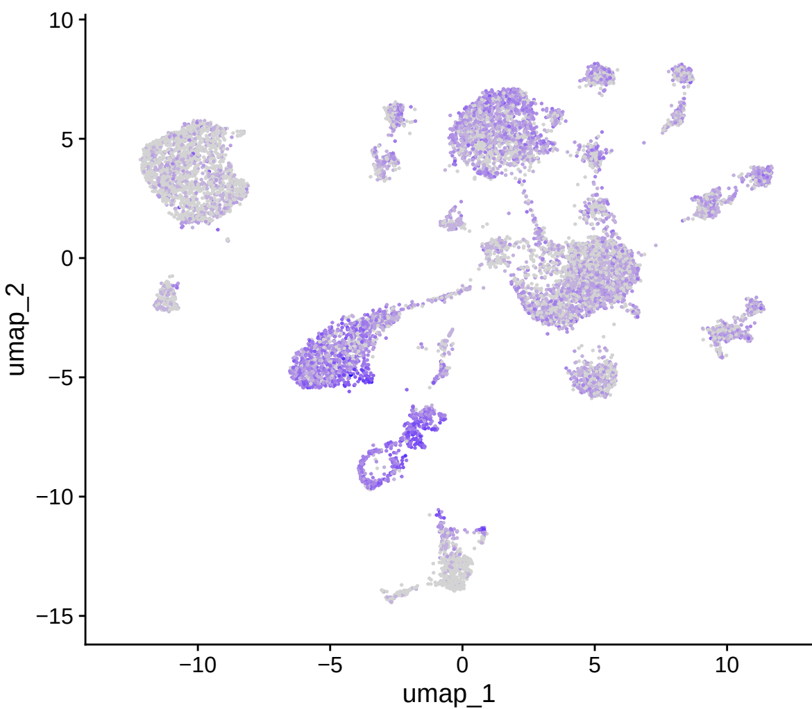
CD79B
