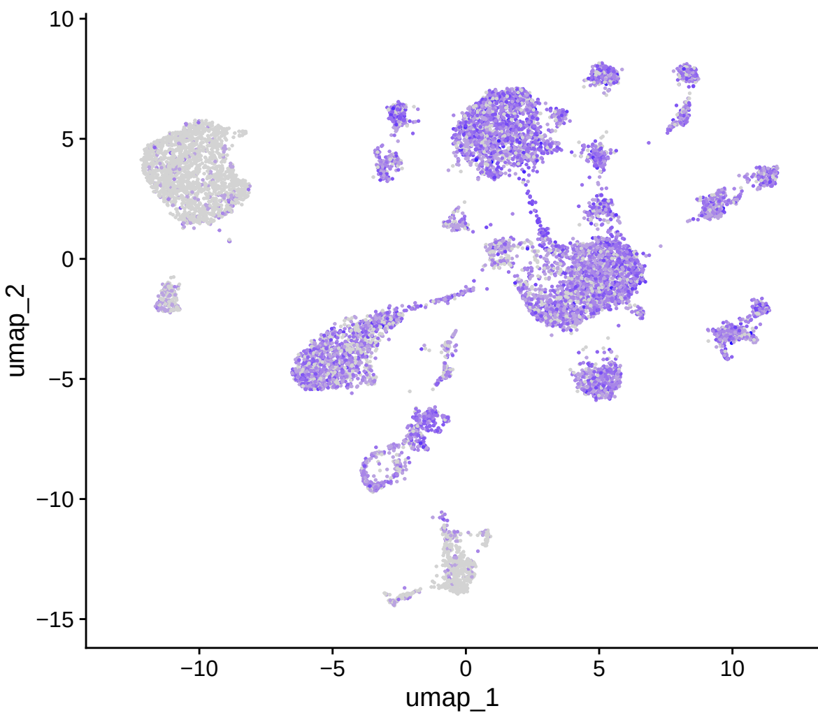
CD79B
