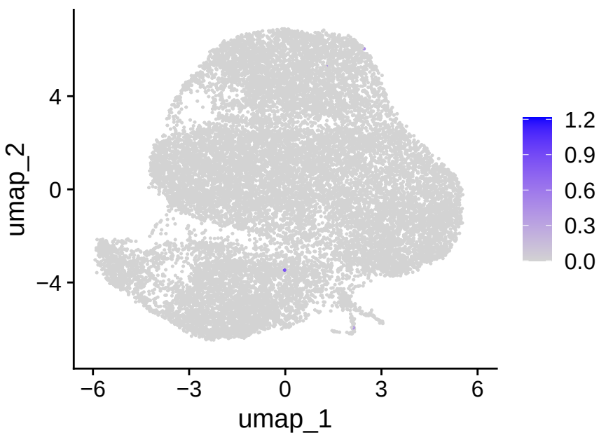
CD7
