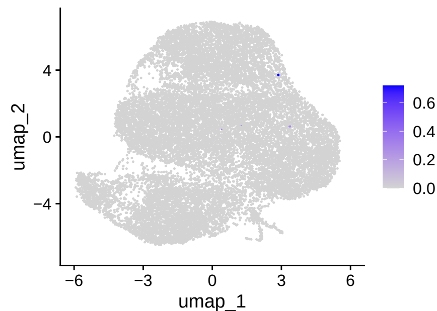
CD8B
