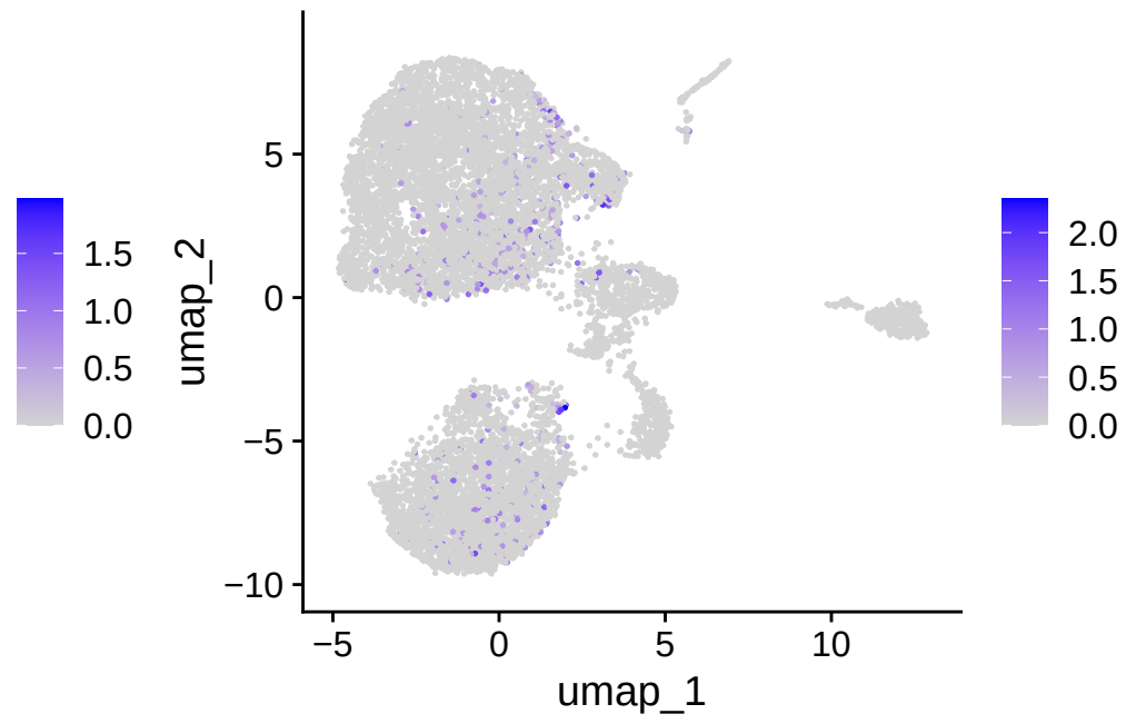
TOP2A
