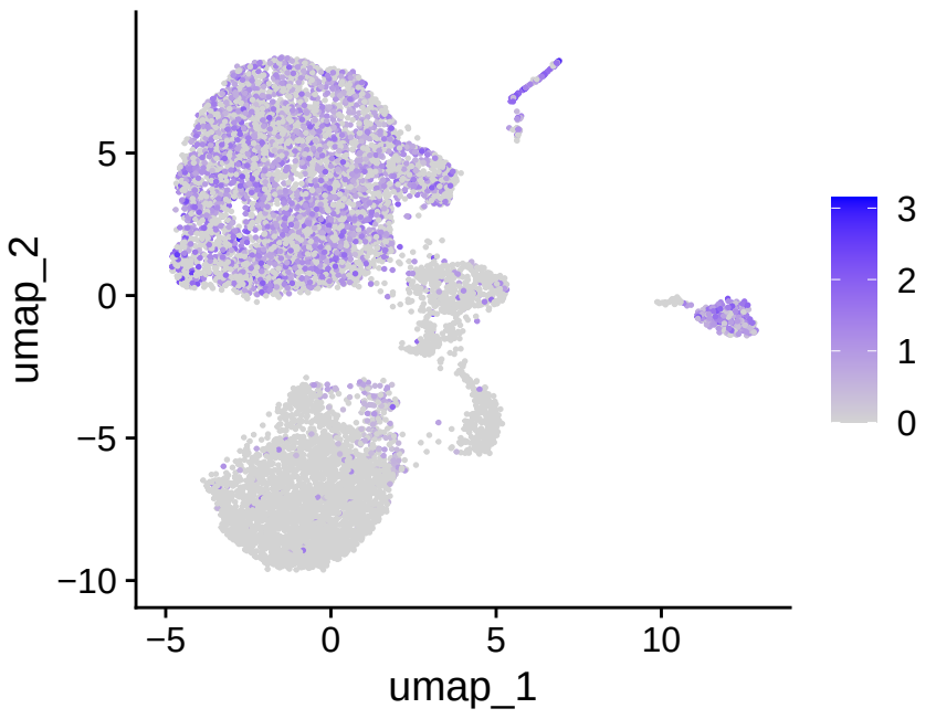
MKI67
