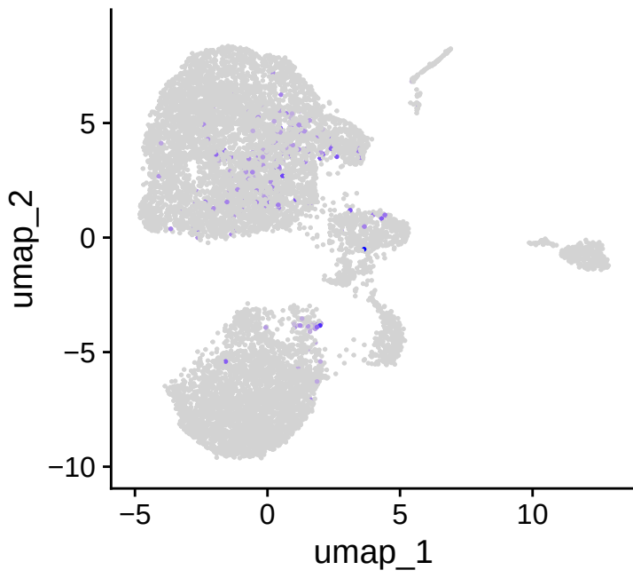
MEF2B
