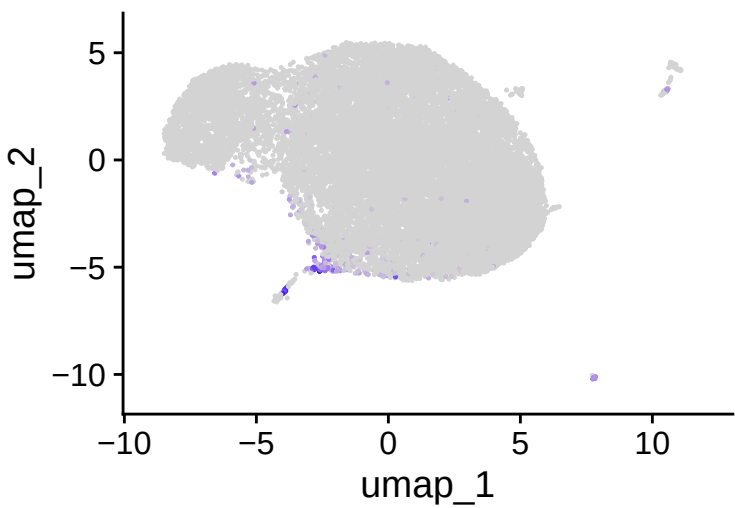
HLA-DPB1
