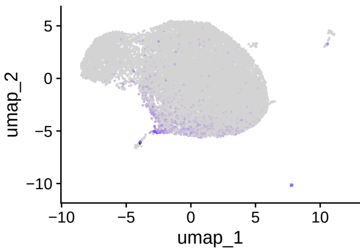
HLA-DQB1
