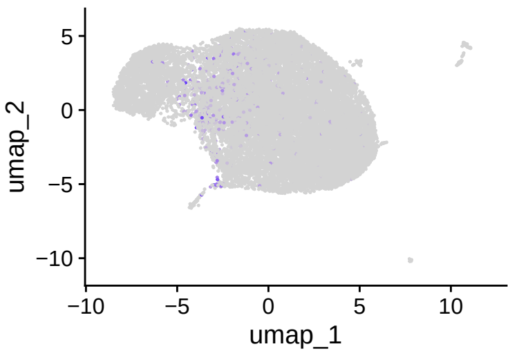
CCR7
