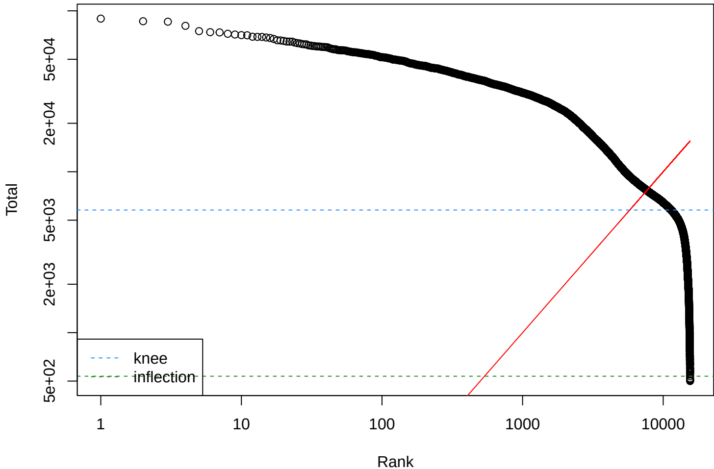
HH117-SI-MILF-nonINF-HLADR-AND-CD19 roughQC-filtered Barcode Rank Plot
