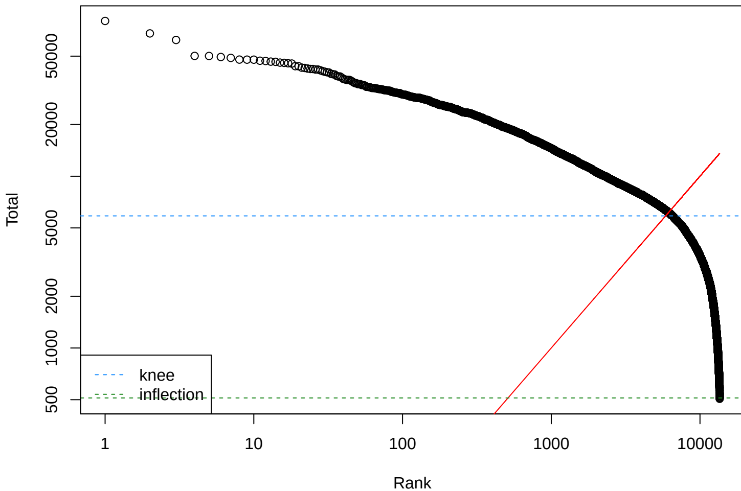
HH119-SI-PP-CD19-Pool1 roughQC-filtered Barcode Rank Plot
