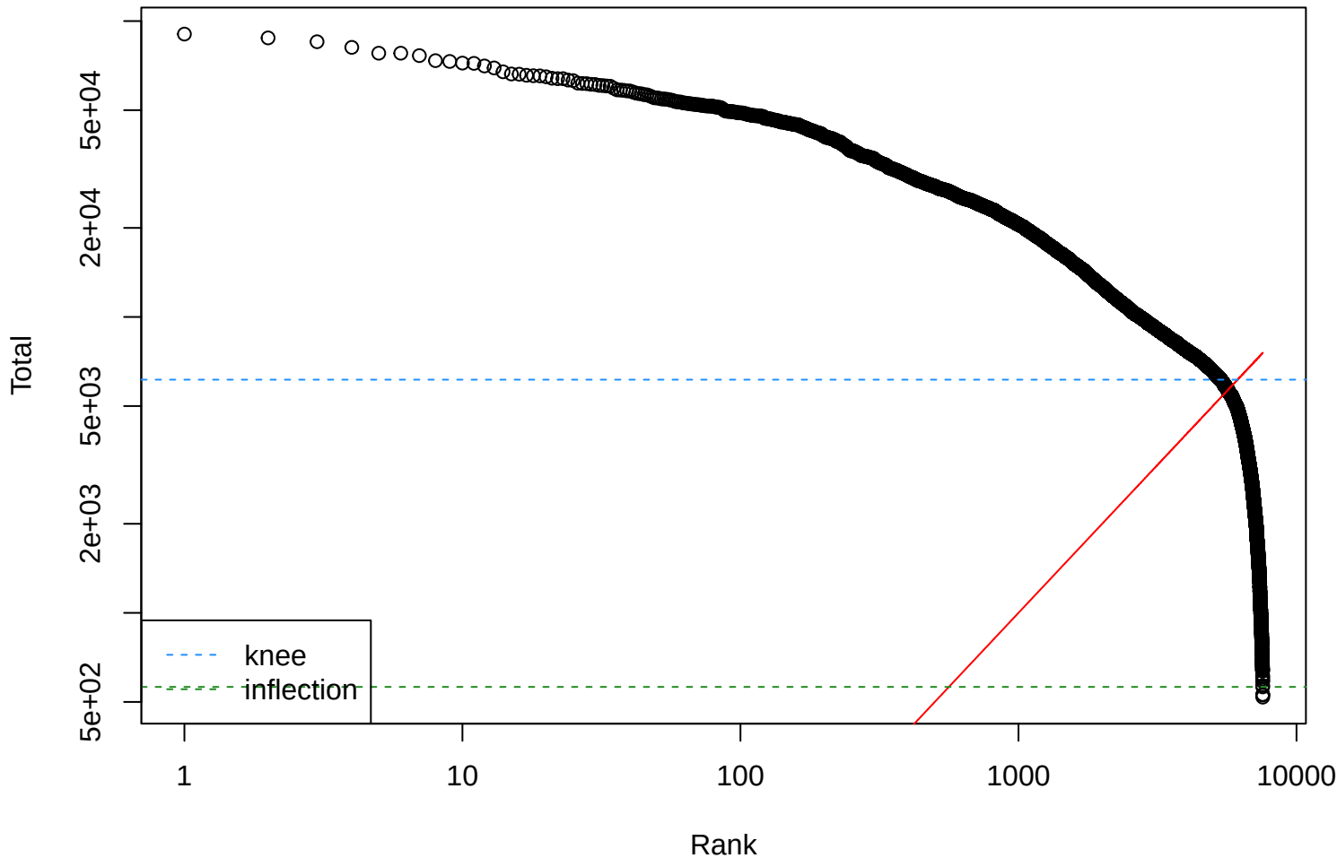
HH119-SI-PP-GC-AND-PB-AND-TFH-Pool1 roughQC-filtered Barcode Rank Plot
