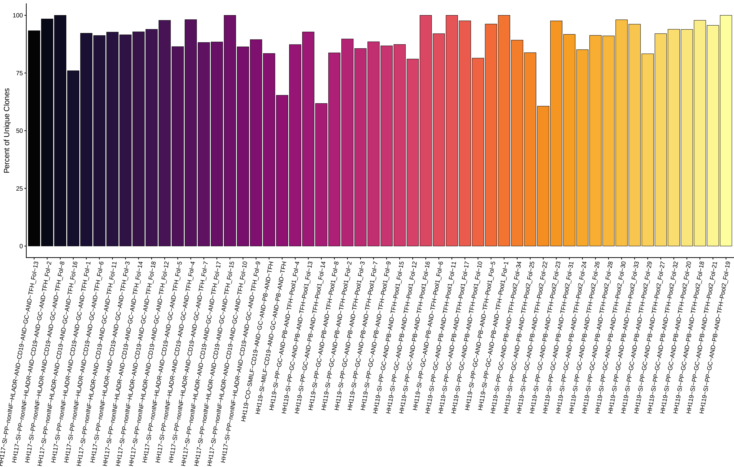
TCR: Relative numbers of unique clones
