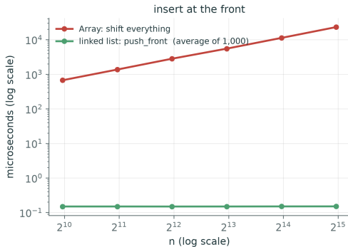
Figure: Real timings, reference implementations on the course Array and on nodes.
