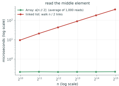
Figure: Real timings, reference implementations on the course Array and on nodes.
