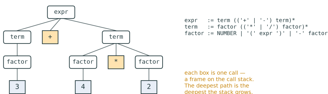
Recursive descent on 3 + 4 * 2 : the calls form a tree (the parse tree)
