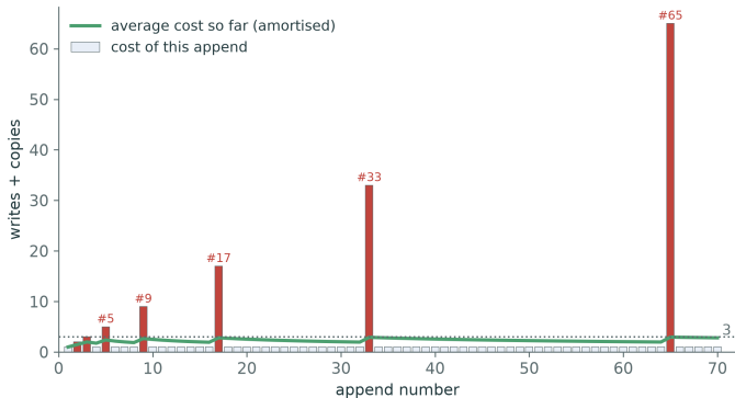
Doubling: a few expensive appends, spread thinly over many cheap ones
