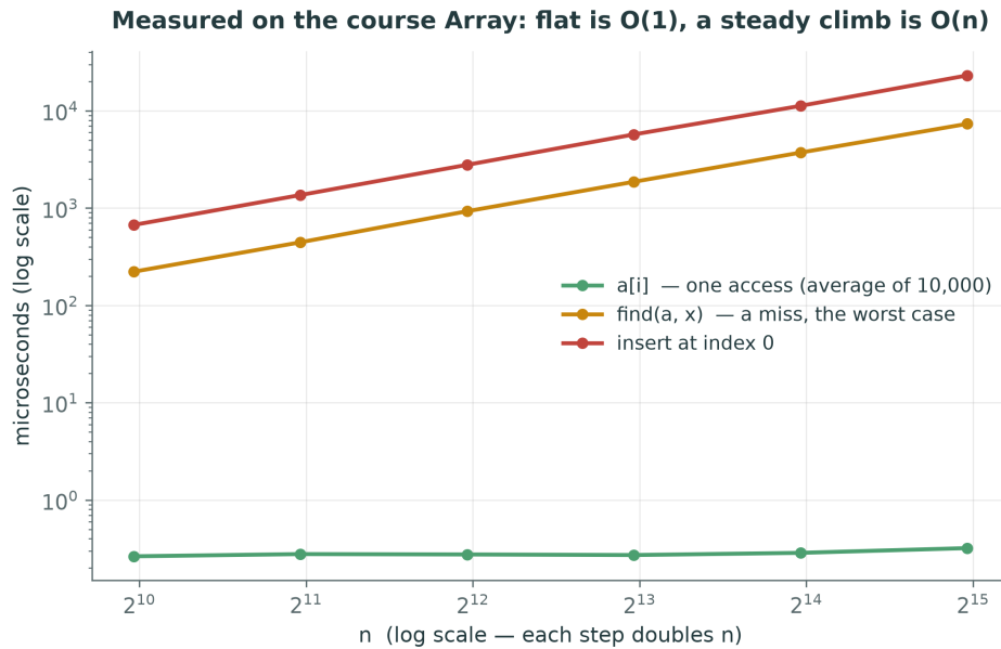
Figure 3: Real timings on the course Array. Each step right doubles n.
