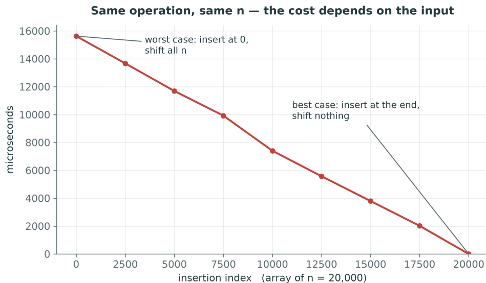
Figure 2: Insertion into an array of 20,000 elements, at nine different positions. Real timings on the course Array.
