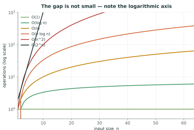
Figure 1: The same curves as Lecture 01. Note the logarithmic vertical axis.
