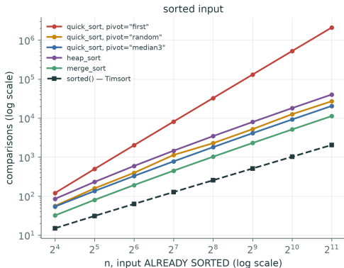
Measured: comparisons made by the six sorts of dsa/sorting.py
