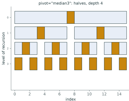
Quicksort on the sorted list 0..14: the pivot decides the shape (amber = pivot's final place)
