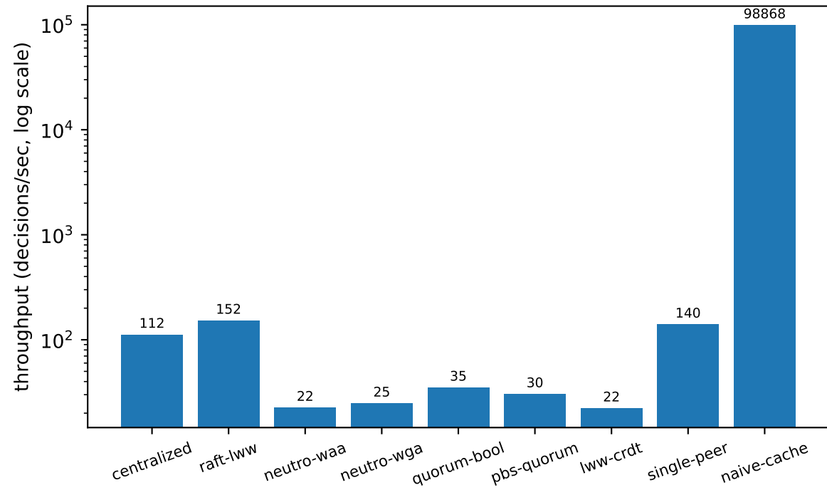
Measured throughput under concurrent load (real HTTP testbed)
