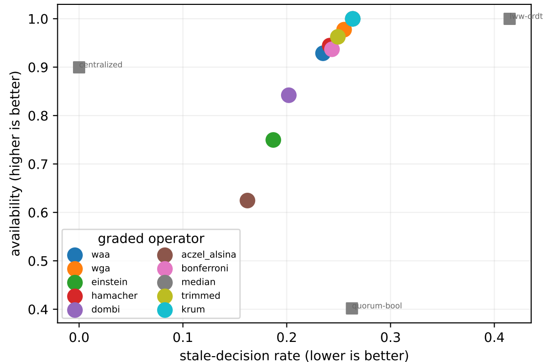
Operator panel spreads the frontier (S2, \phi=0.1 )
