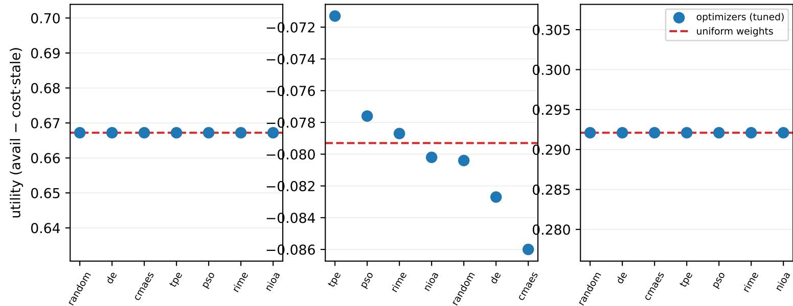
Axis-B: tuning is optimizer-agnostic; it beats uniform weights only under asymmetric cost (S2)
