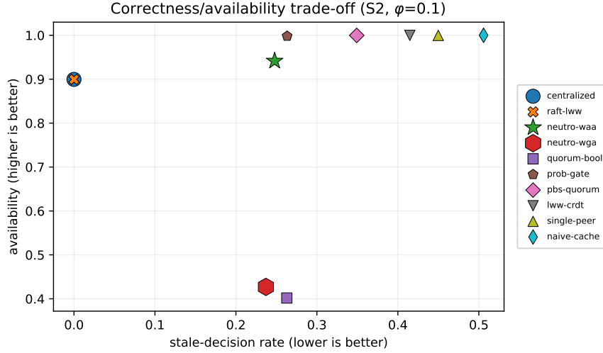
Figure 1: Correctness/availability trade-off (S2, \varphi = 0.1 ). Up-and-left is better; neutro-waa is on the Pareto frontier. Each system has a distinct marker; the strongly-consistent baselines centralized and raft-lww coincide at (0, 0.90) (circle behind cross).
