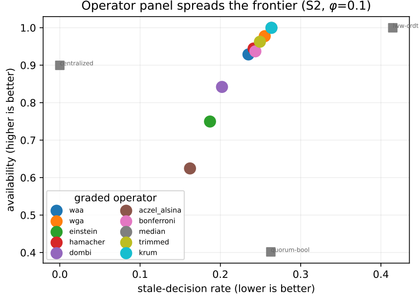
Figure 3: Axis A: the graded operator panel spreads a tunable correctness/availability frontier at fixed \tau (S2, \varphi = 0.1 ), from conservative (Aczél–Alsina) to optimistic (median/Krum), bracketed by the consistency baselines. On crisp inputs every operator collapses to WAA.
