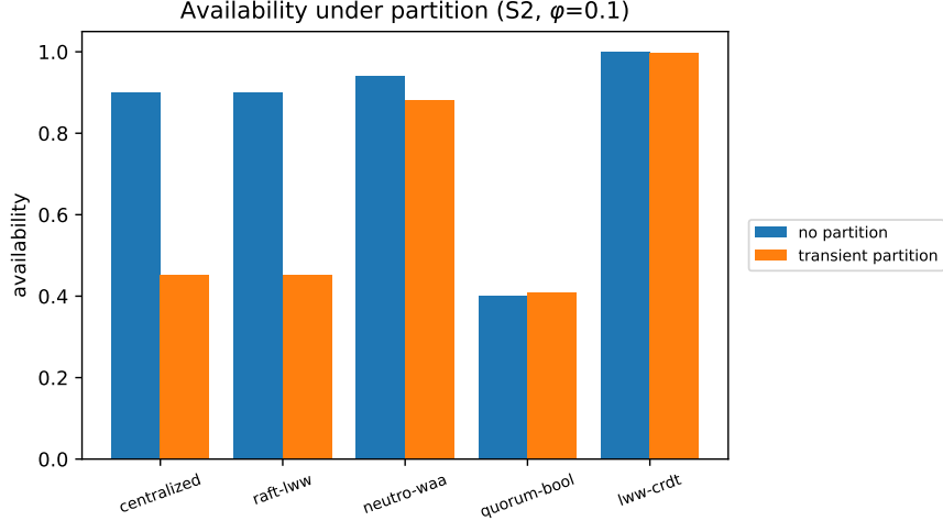
Figure 2: Availability without vs. with transient partition (S2, \varphi = 0.1 ). The strongly-consistent baselines stall; the neutrosophic layer stays available.
