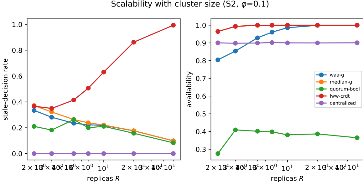
Figure 5: Scalability with replica count R (S2, \varphi = 0.1 ): the neutrosophic layer’s stale-rate falls and availability rises with R (at R messages/decision), whereas eventual consistency degrades with scale and the boolean quorum stays low-availability.
