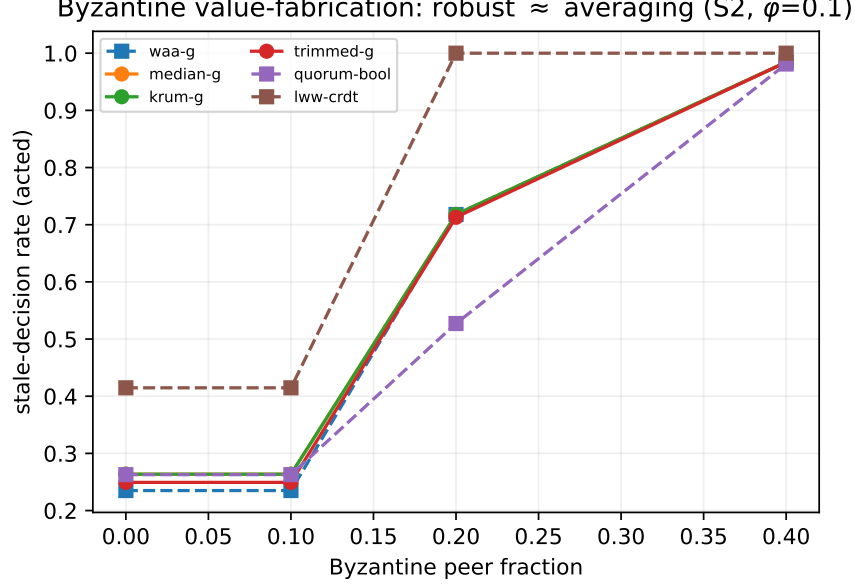
Figure 4: Byzantine value-fabrication (S2, \varphi = 0.1 , R = 5 ): the robust aggregators (median, Krum, trimmed mean) degrade together with the averaging operators as the adversary fraction grows—robust aggregation defends the gate (Lemma 3), not value selection.
